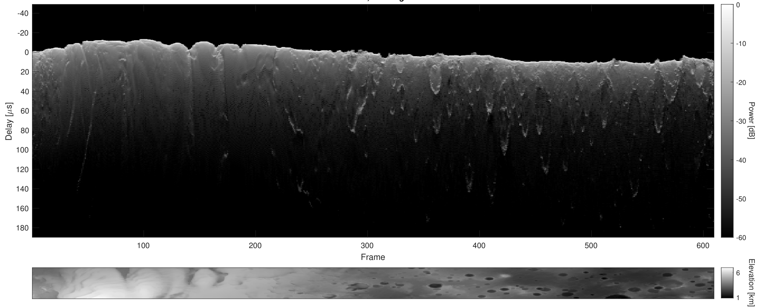
Orbit 6393, Cluttergram
