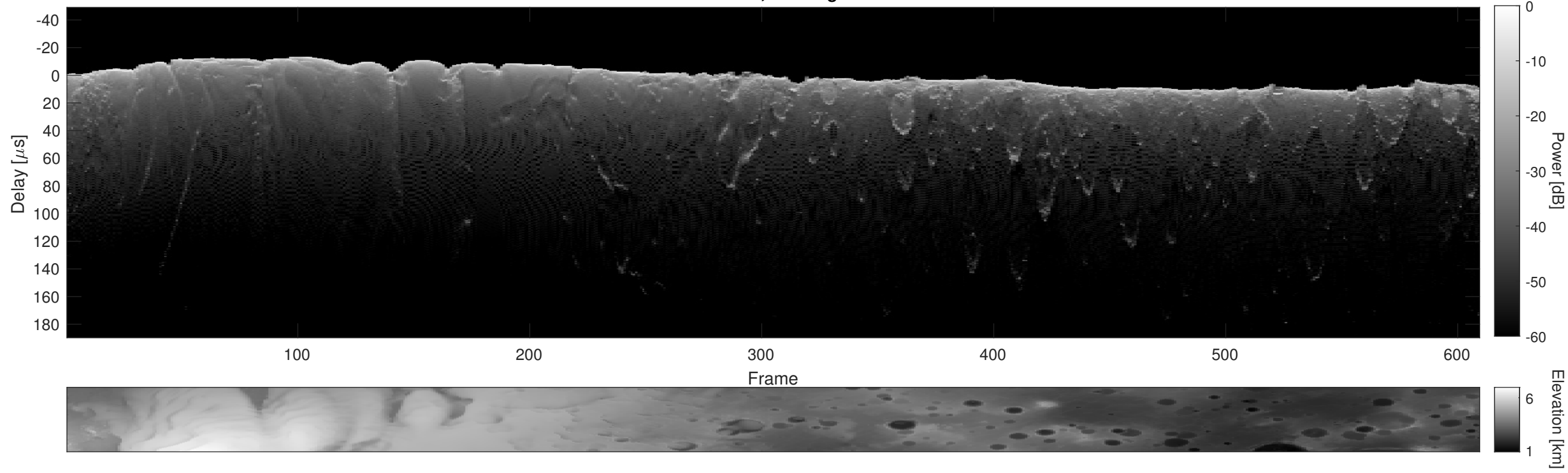
Orbit 6393, Cluttergram
