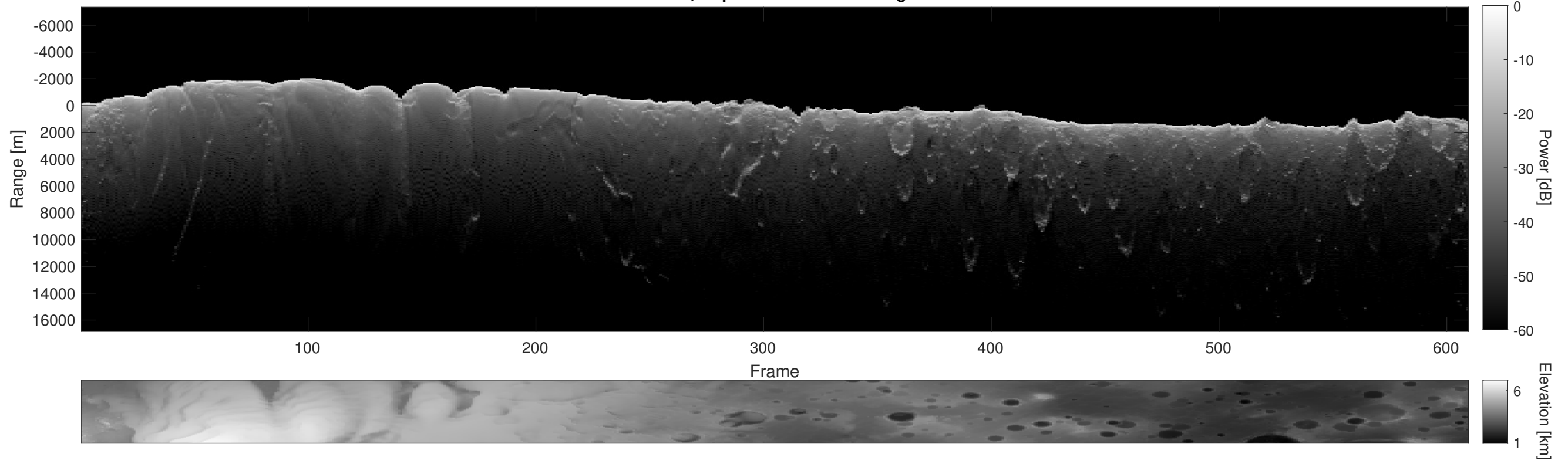
Orbit 6393, Depth-Corrected Cluttergram
