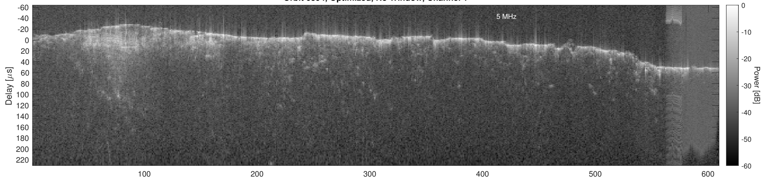
Orbit 6394, Optimized, No Window, Channel 2
