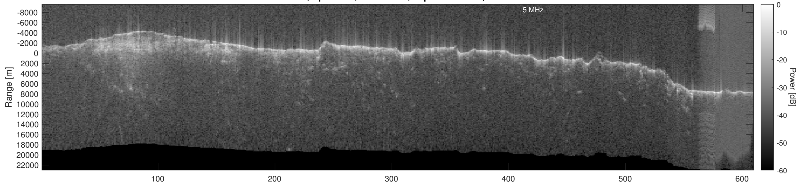
Orbit 6394, Optimized, No Window, Depth-Corrected, Channel 2
