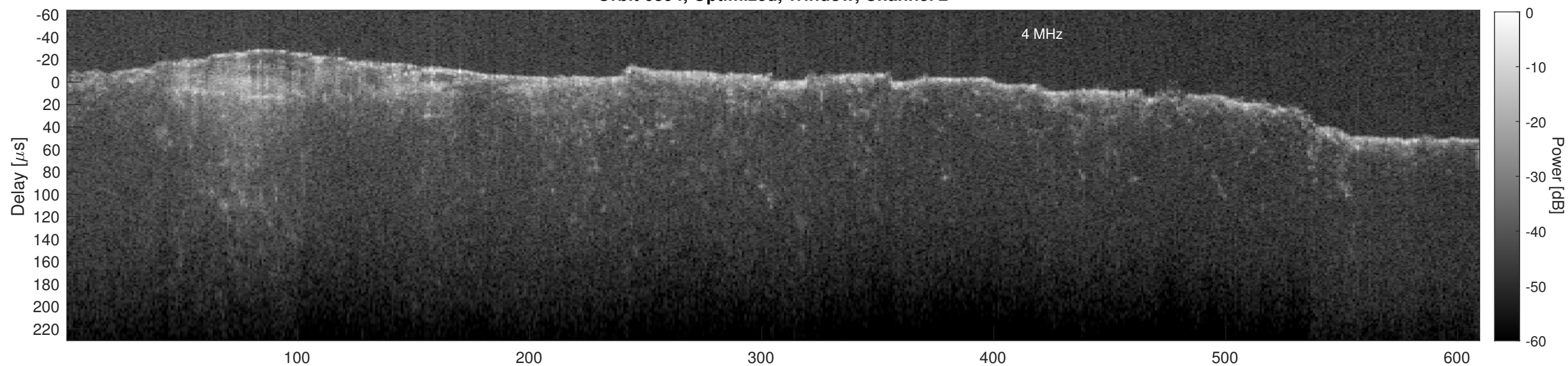
Orbit 6394, Cluttergram
