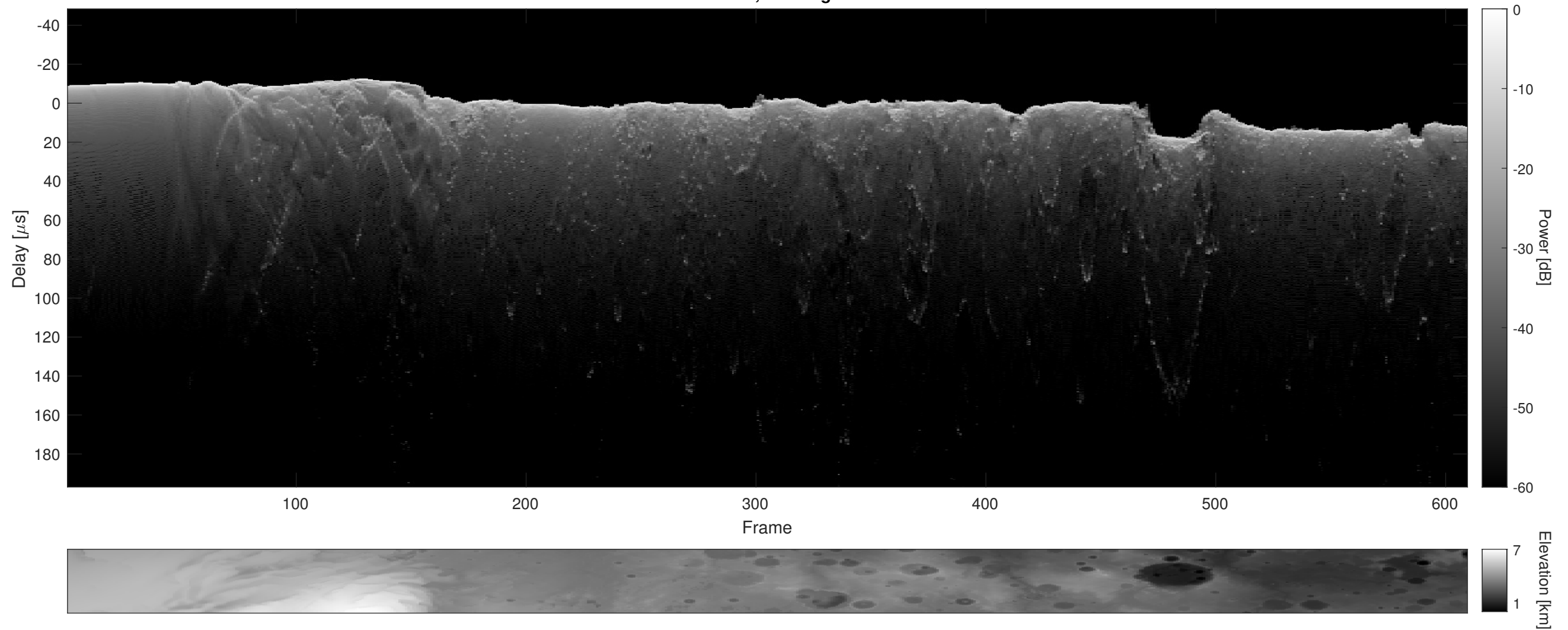
Orbit 6395, Cluttergram
