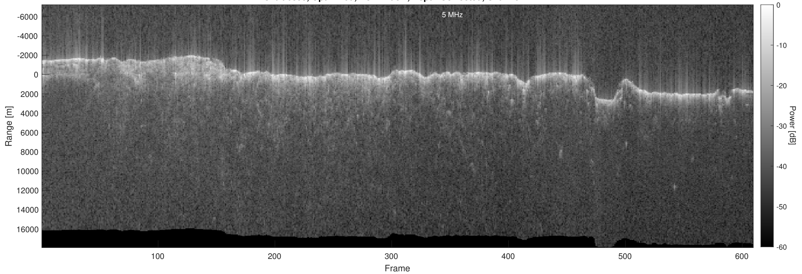
Orbit 6395, Optimized, No Window, Depth-Corrected, Channel 2
