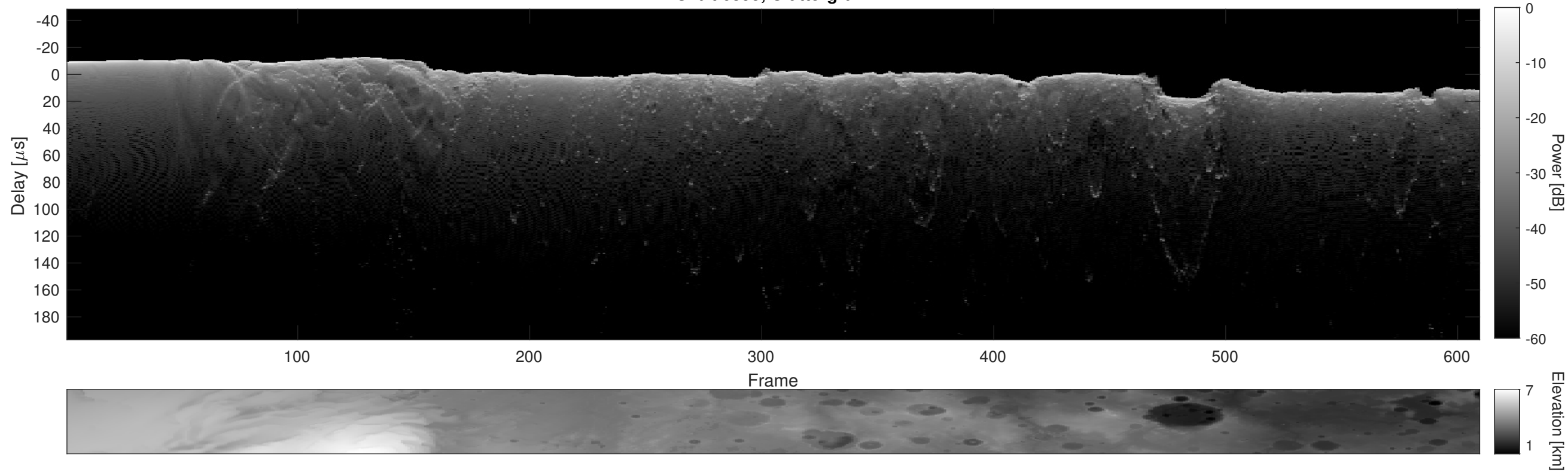
Orbit 6395, Cluttergram
