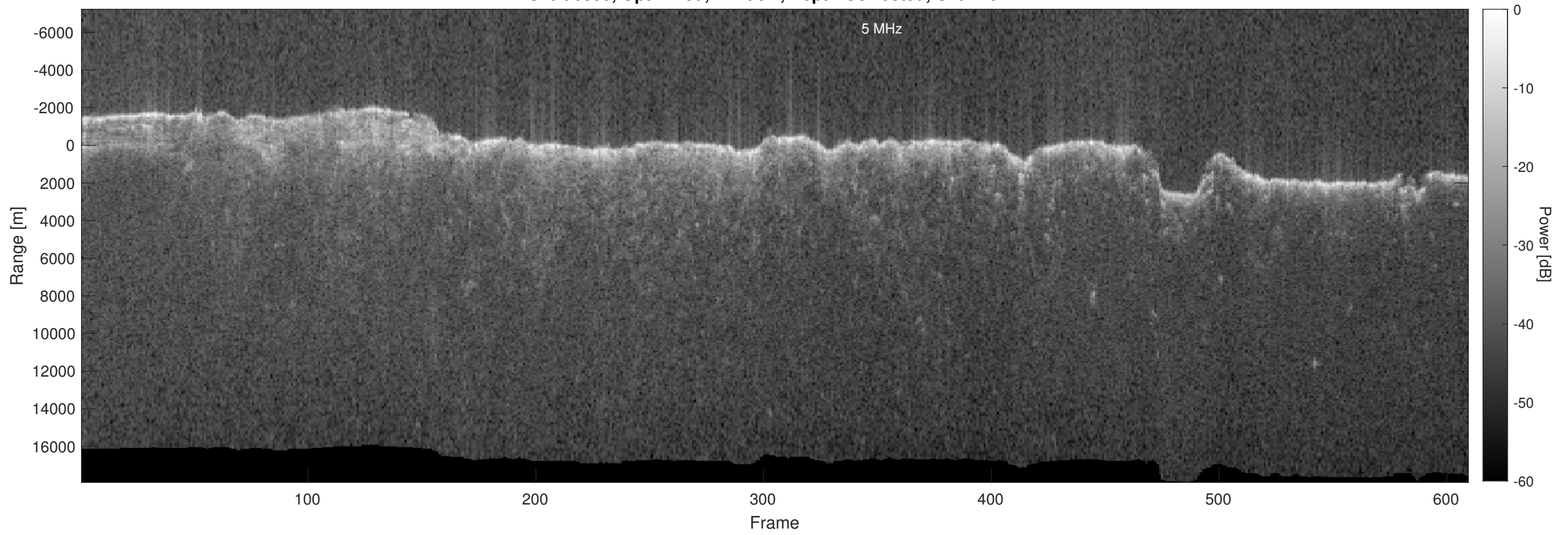
Orbit 6395, Optimized, Window, Depth-Corrected, Channel 2
