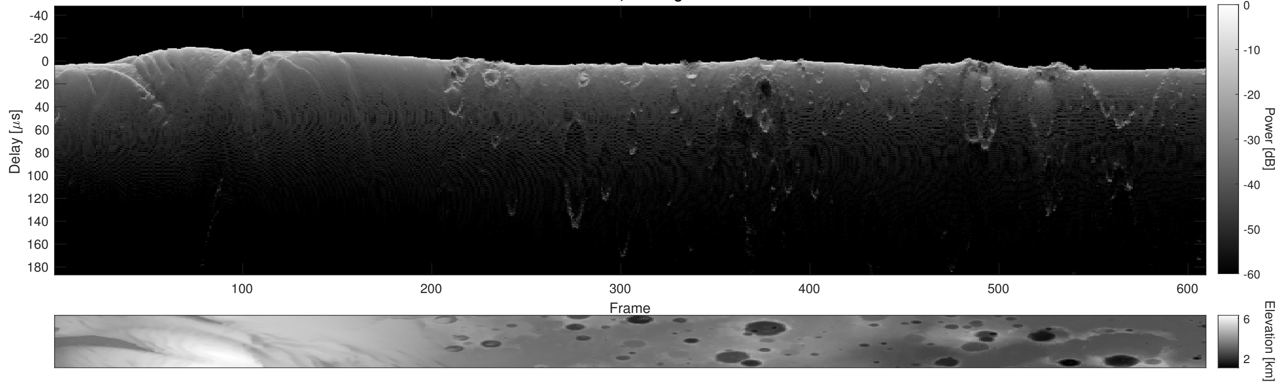
Orbit 6396, Cluttergram
