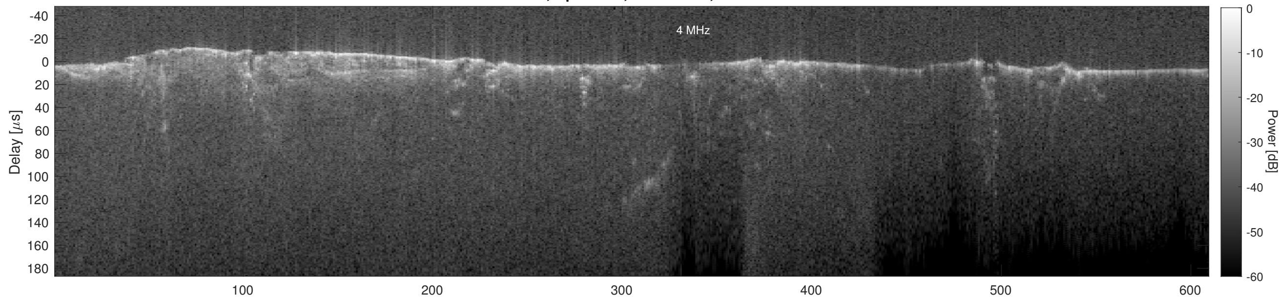
Orbit 6396, Cluttergram
