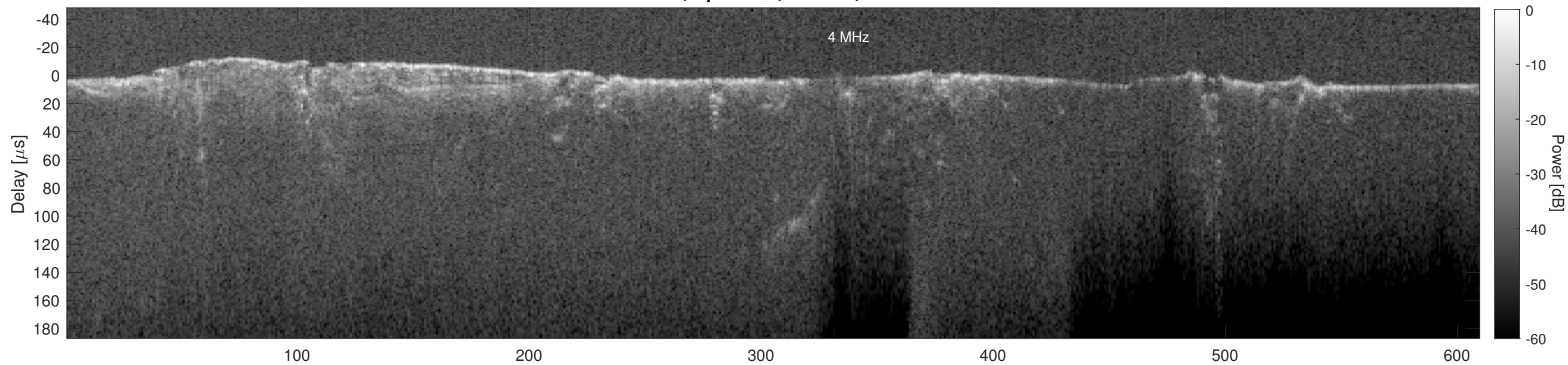
Orbit 6396, Cluttergram
