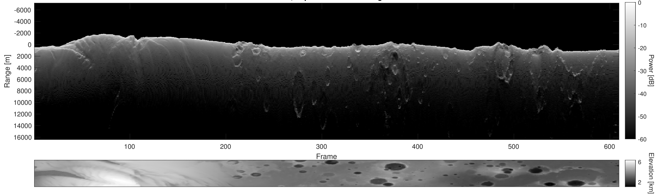
Orbit 6396, Depth-Corrected Cluttergram
