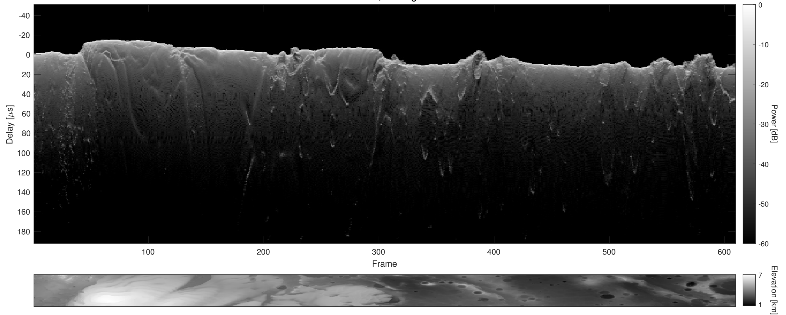
Orbit 6397, Cluttergram
