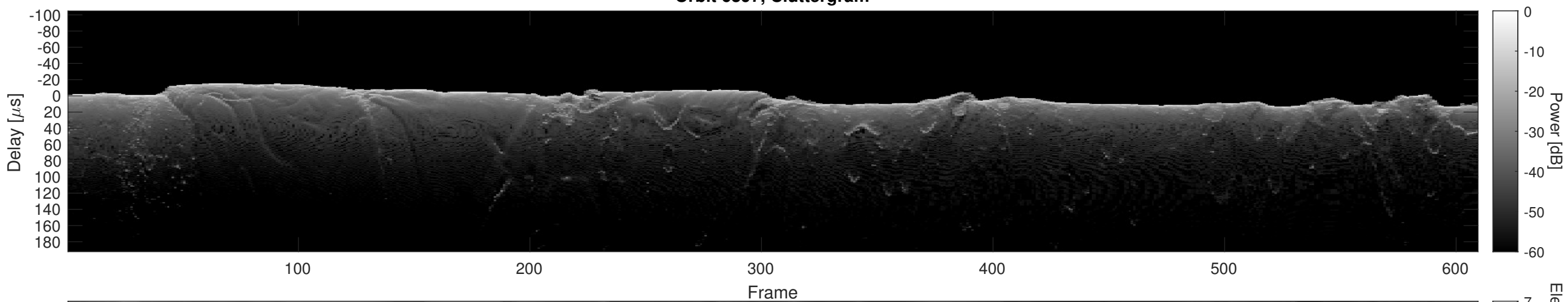
Orbit 6397, Cluttergram
