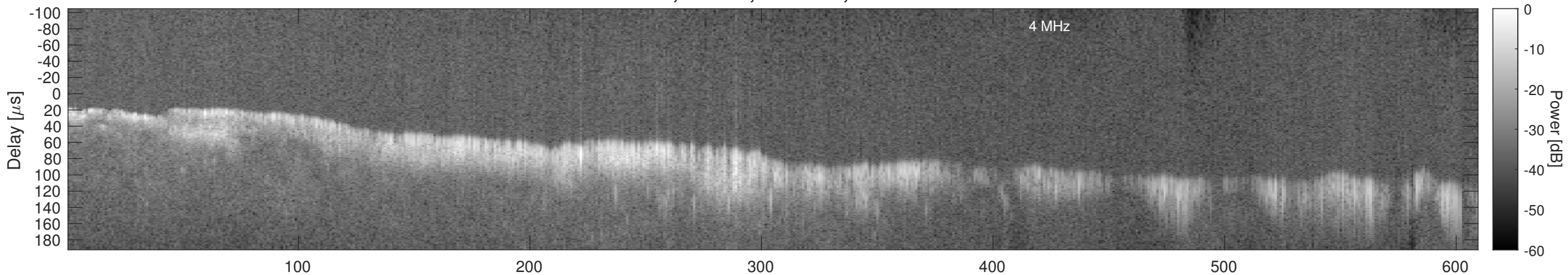
Orbit 6397, Window, Channel 2, Chapman
