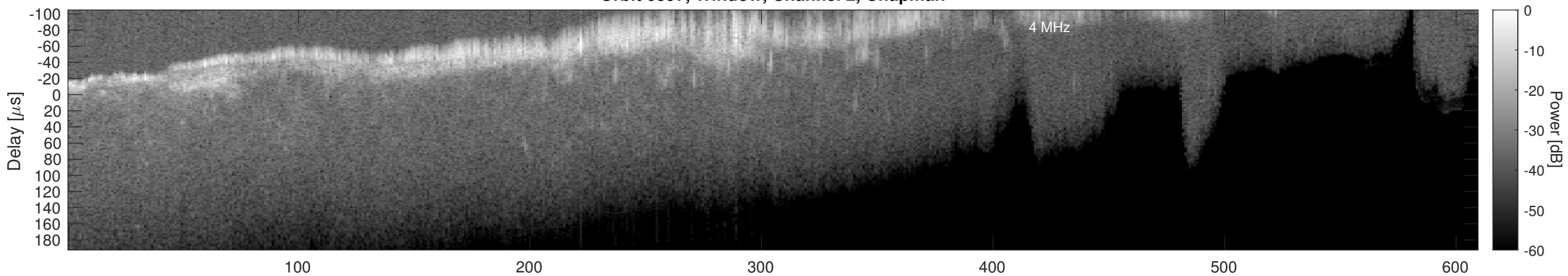
Orbit 6397, Window, Channel 2, Optimized
