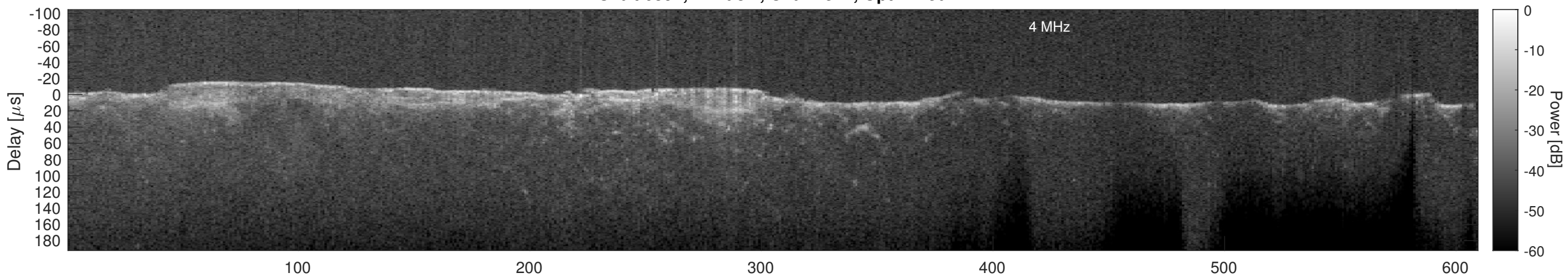
Orbit 6397, Cluttergram
