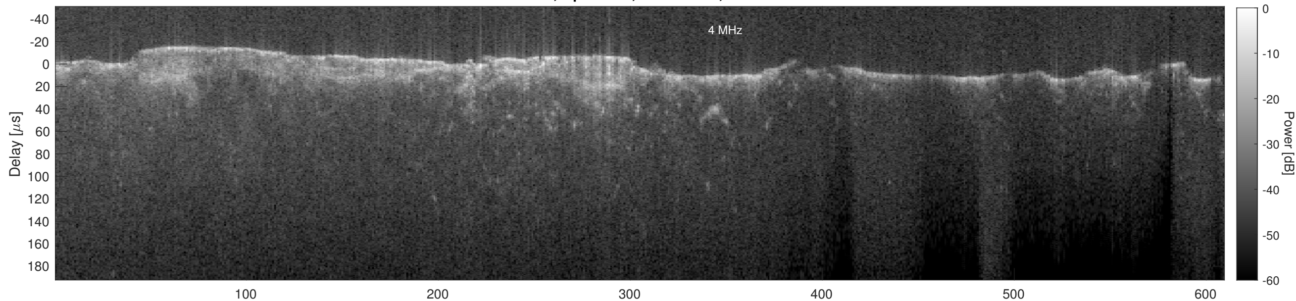
Orbit 6397, Cluttergram
