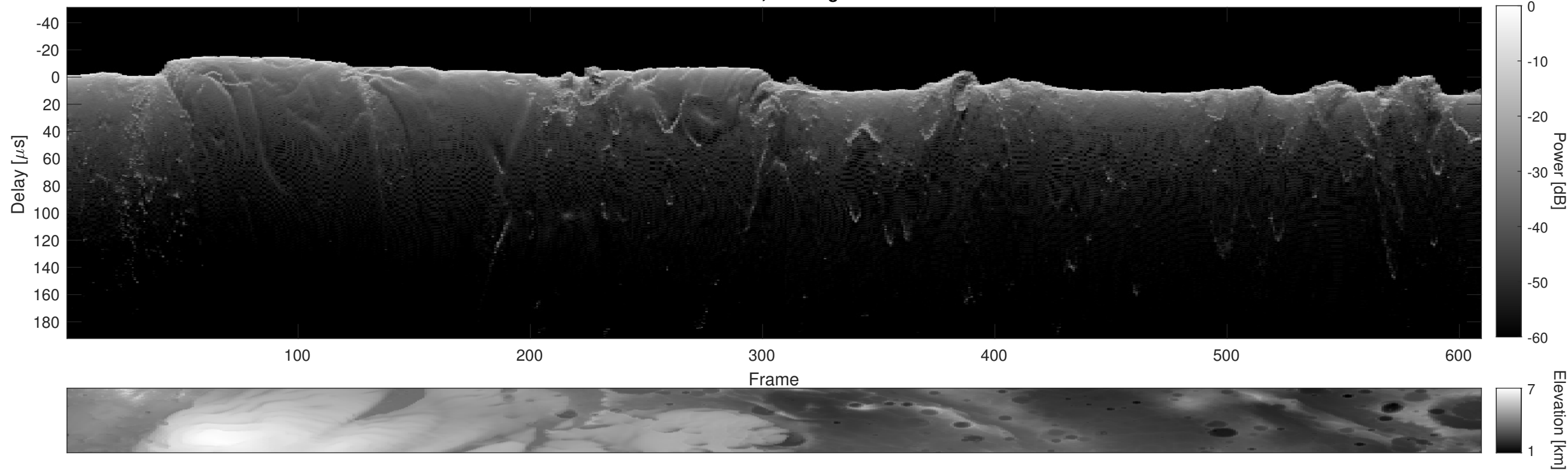
Orbit 6397, Cluttergram
