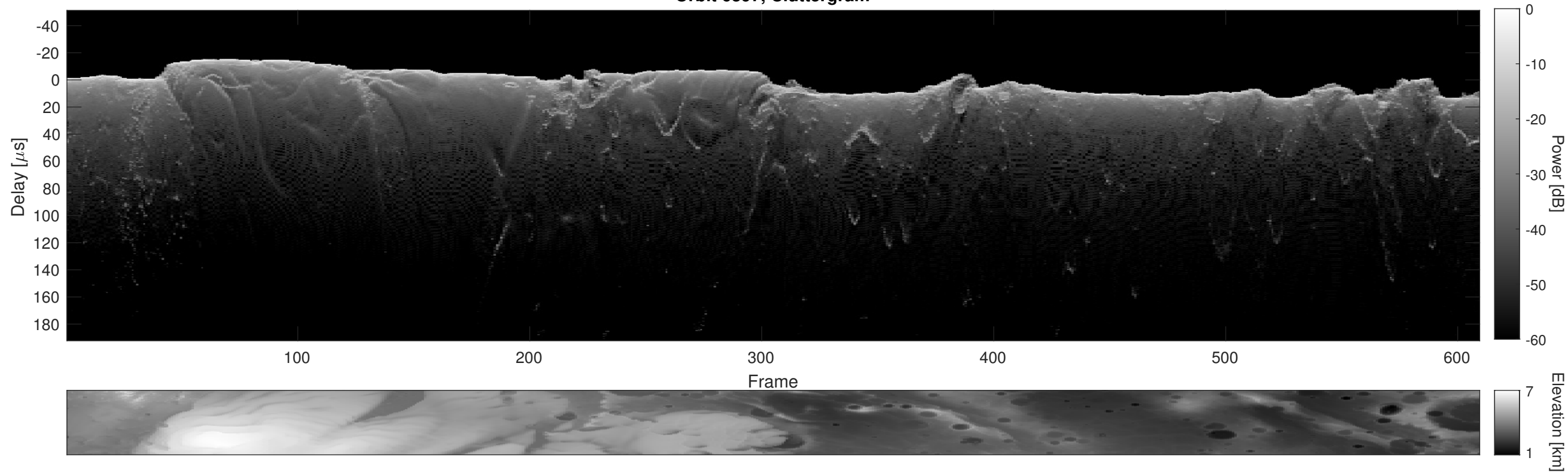
Orbit 6397, Cluttergram
