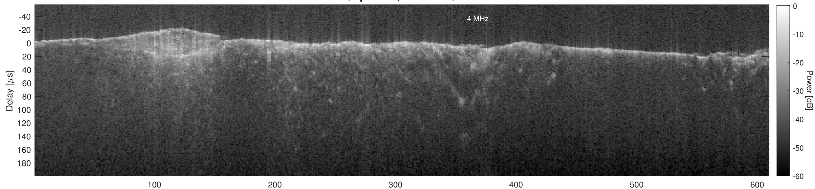
Orbit 6398, Cluttergram
