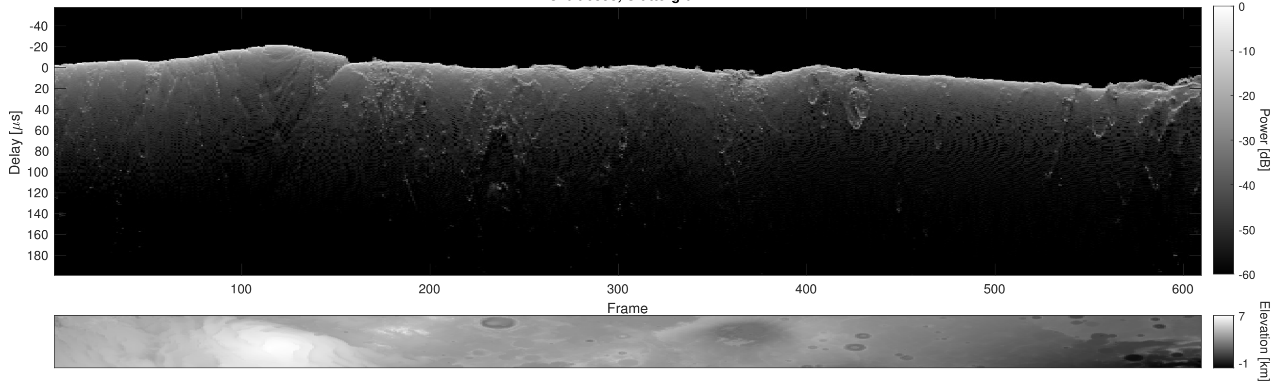
Orbit 6398, Cluttergram
