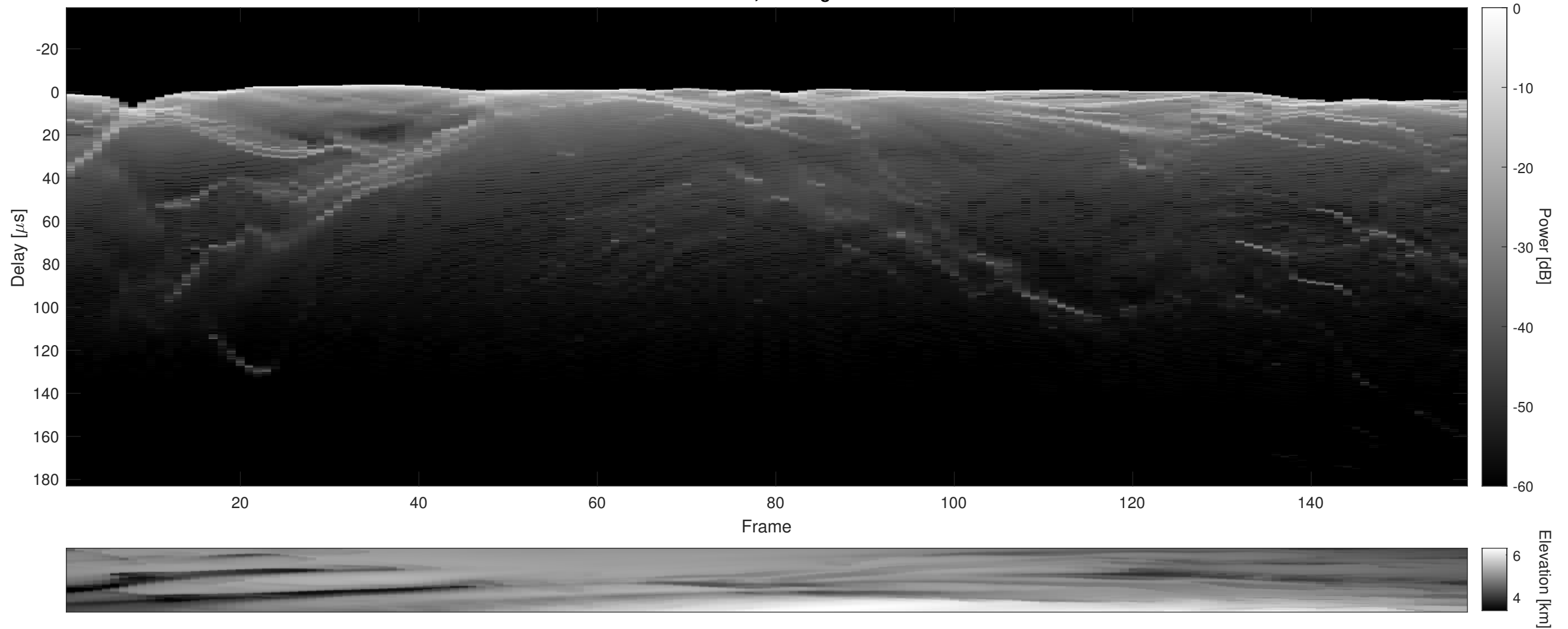
Orbit 6399, Cluttergram
