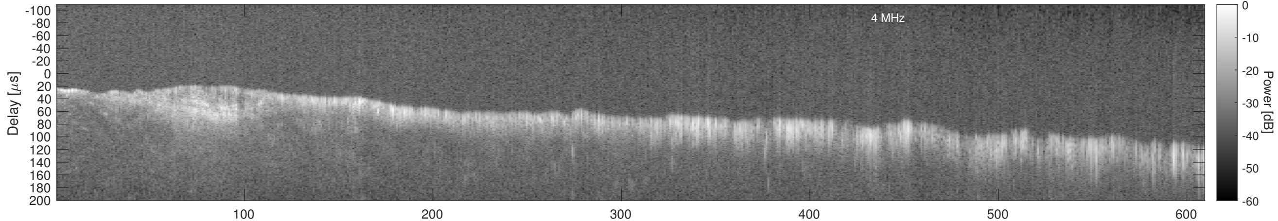
Orbit 6401, Window, Channel 2, Chapman
