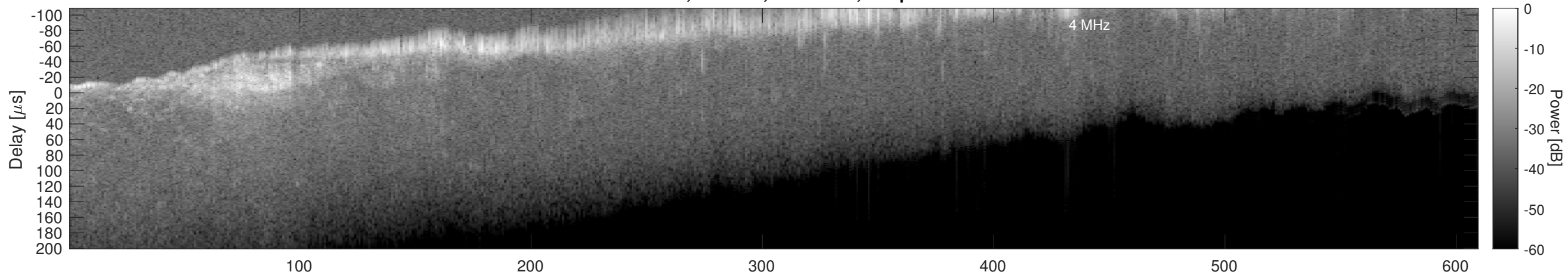
Orbit 6401, Window, Channel 2, Optimized
