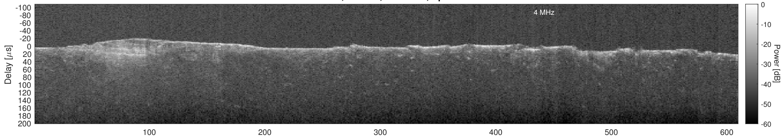
Orbit 6401, Cluttergram
