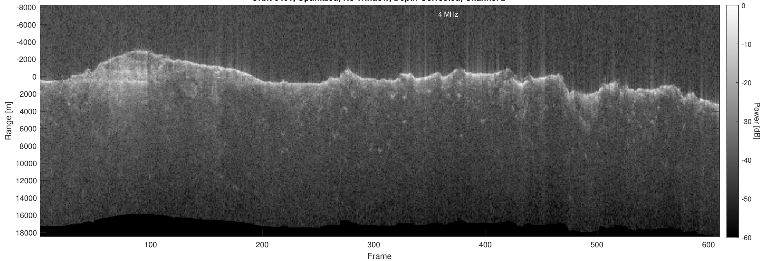
Orbit 6401, Optimized, No Window, Depth-Corrected, Channel 2
