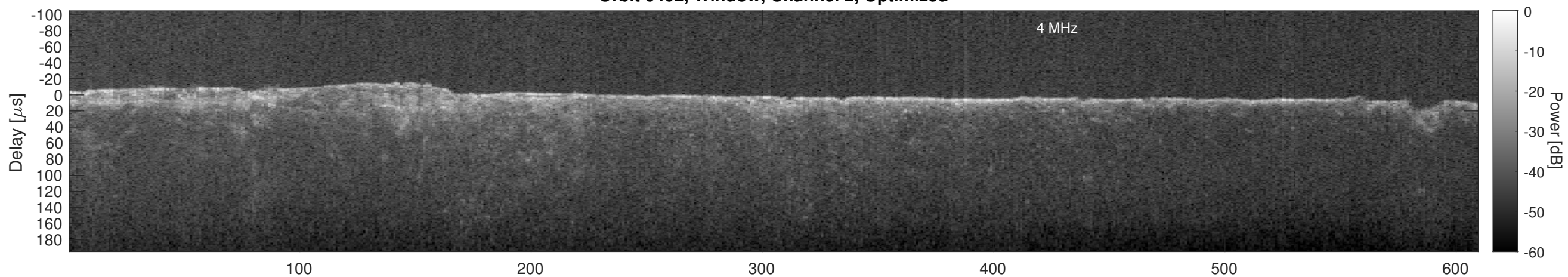
Orbit 6402, Cluttergram
