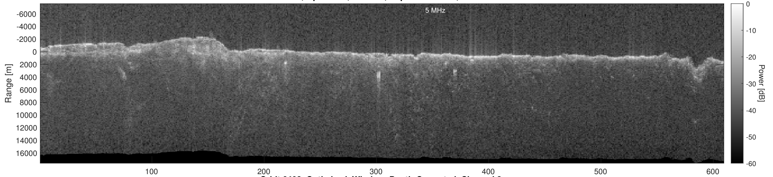
Orbit 6402, Optimized, Window, Depth-Corrected, Channel 2
