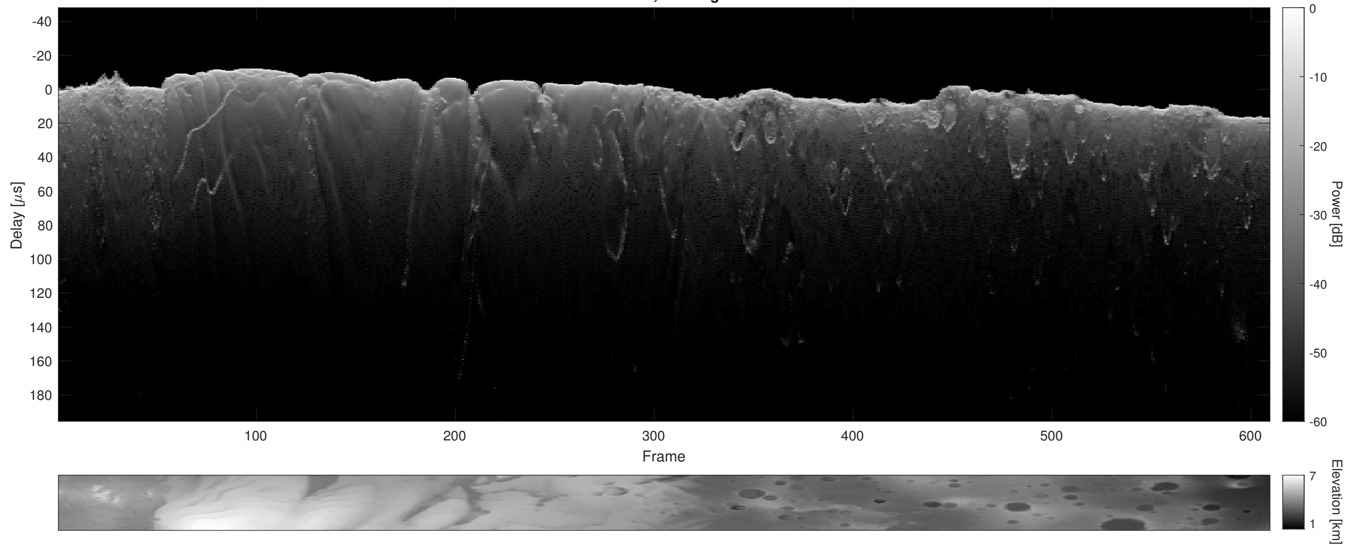
Orbit 6404, Cluttergram
