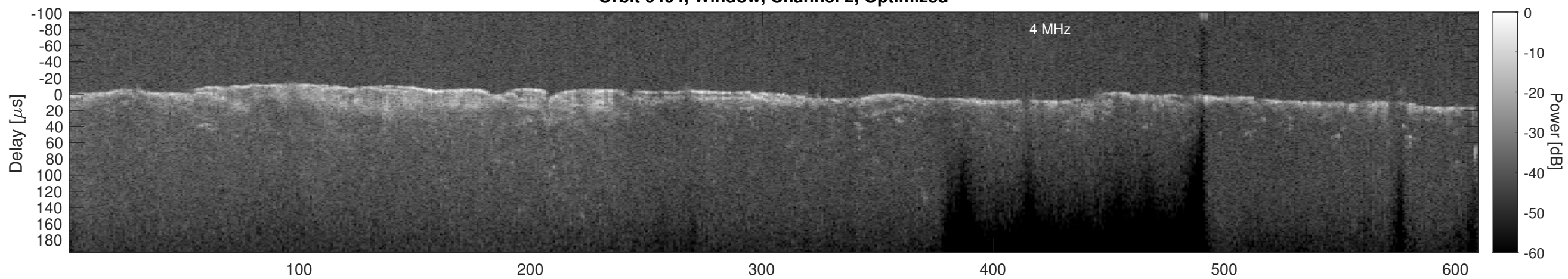
Orbit 6404, Cluttergram
