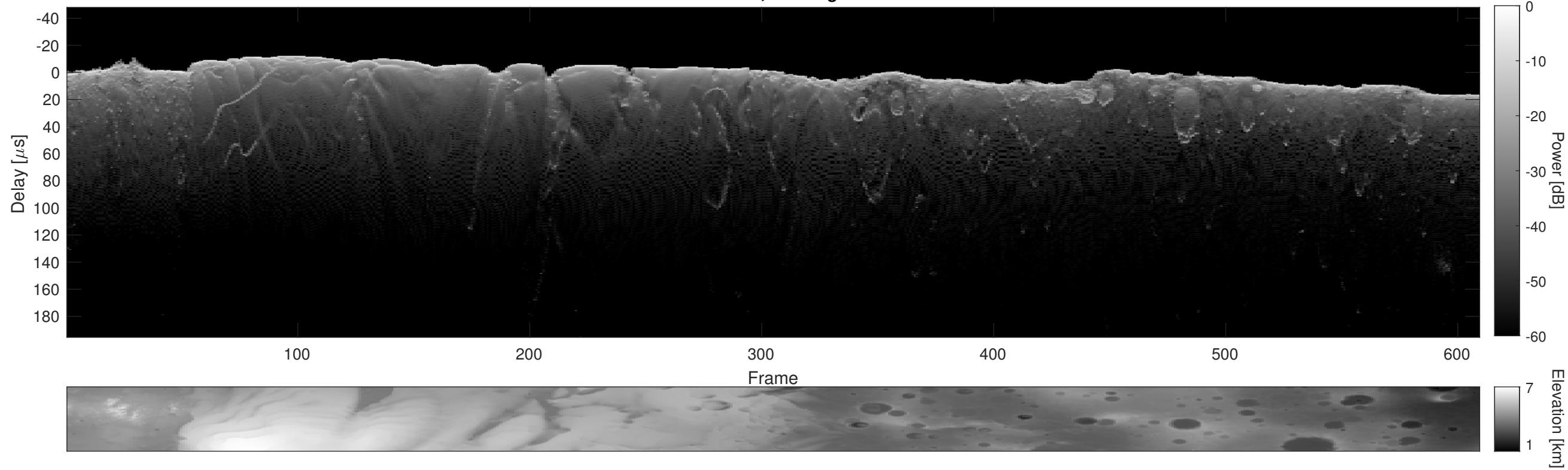
Orbit 6404, Cluttergram
