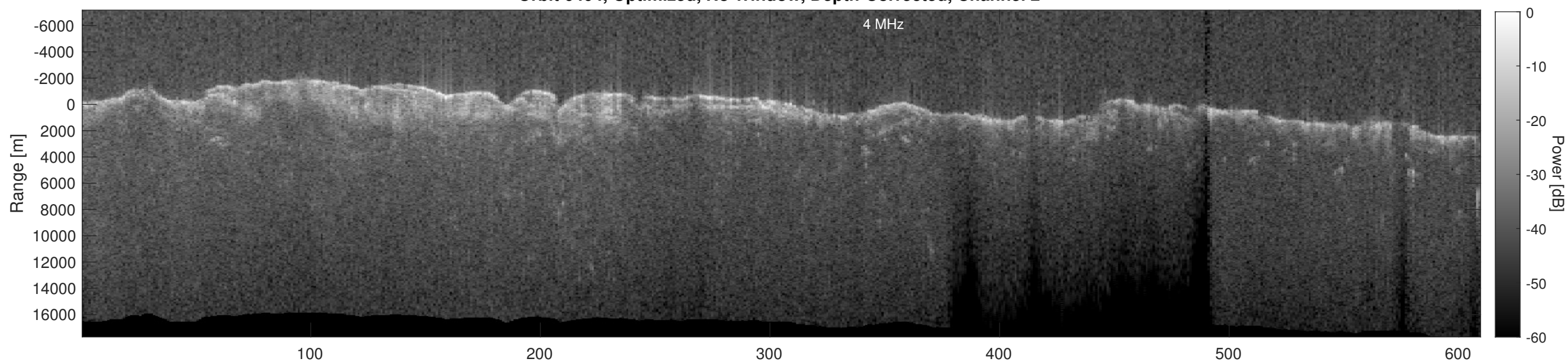
Orbit 6404, Depth-Corrected Cluttergram
