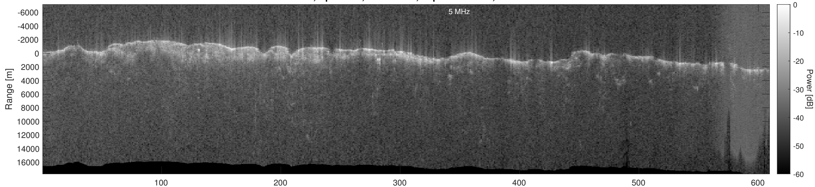
Orbit 6404, Optimized, No Window, Depth-Corrected, Channel 2
