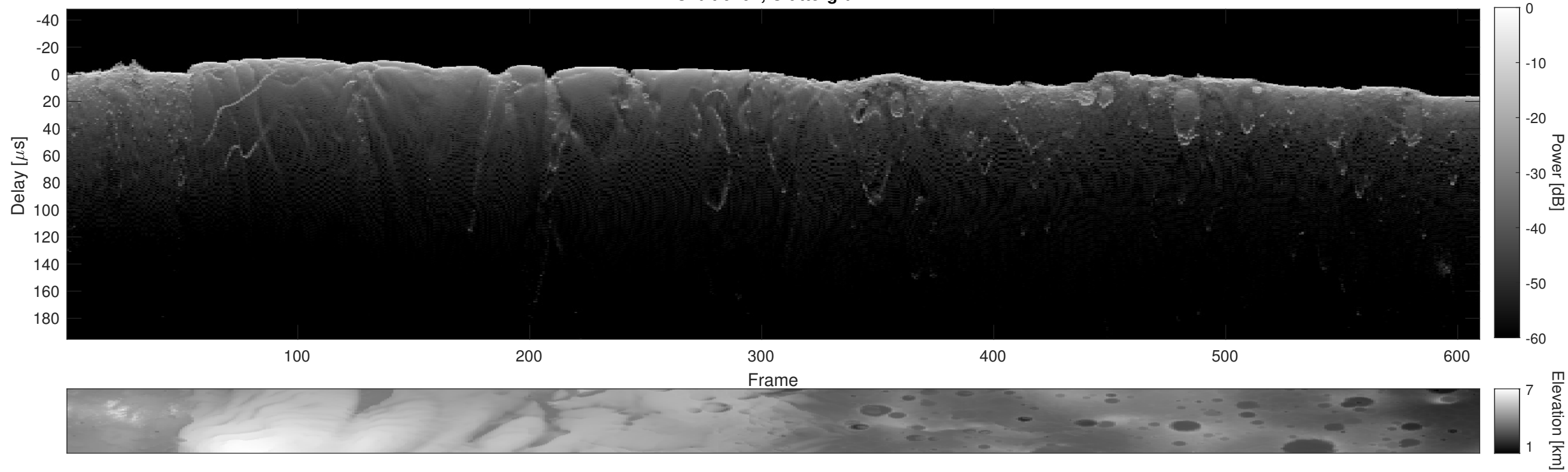
Orbit 6404, Cluttergram
