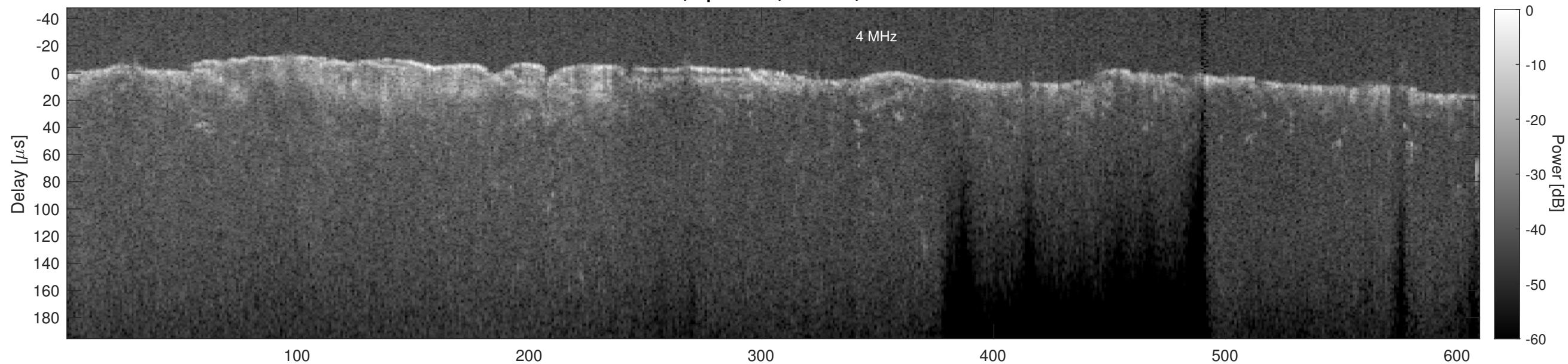
Orbit 6404, Cluttergram
