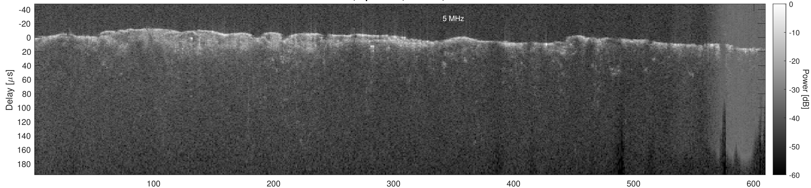
Orbit 6404, Optimized, Window, Channel 2
