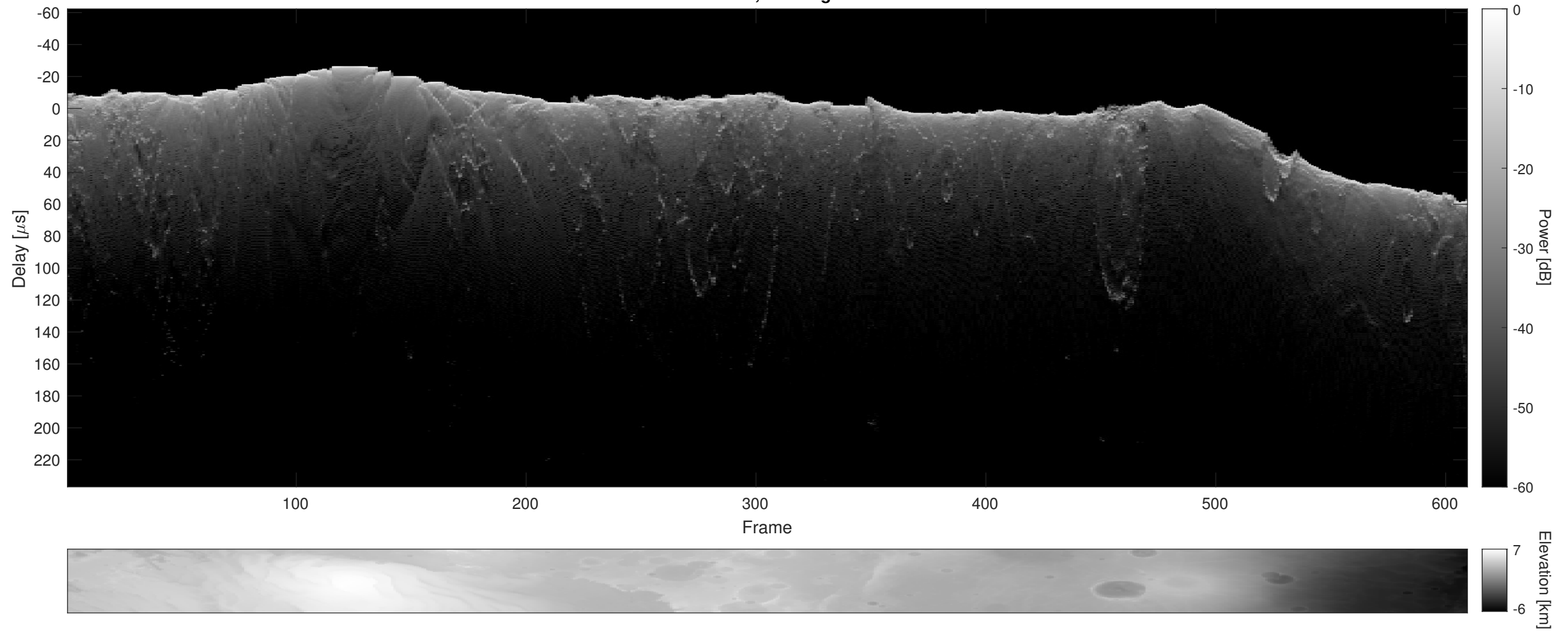
Orbit 6405, Cluttergram
