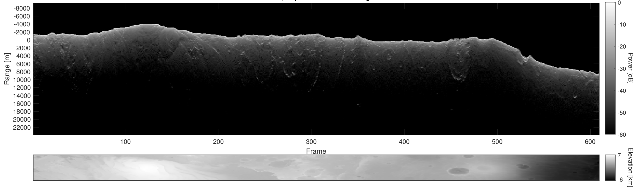
Orbit 6405, Depth-Corrected Cluttergram
