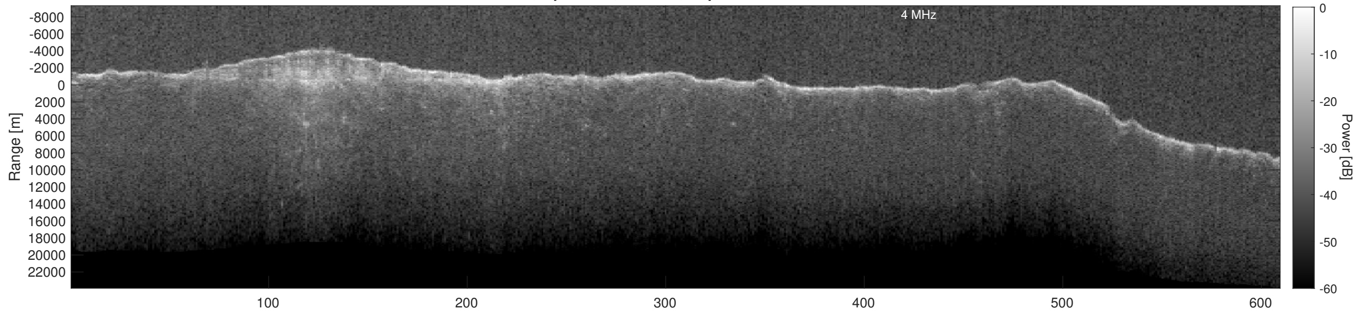
Orbit 6405, Depth-Corrected Cluttergram
