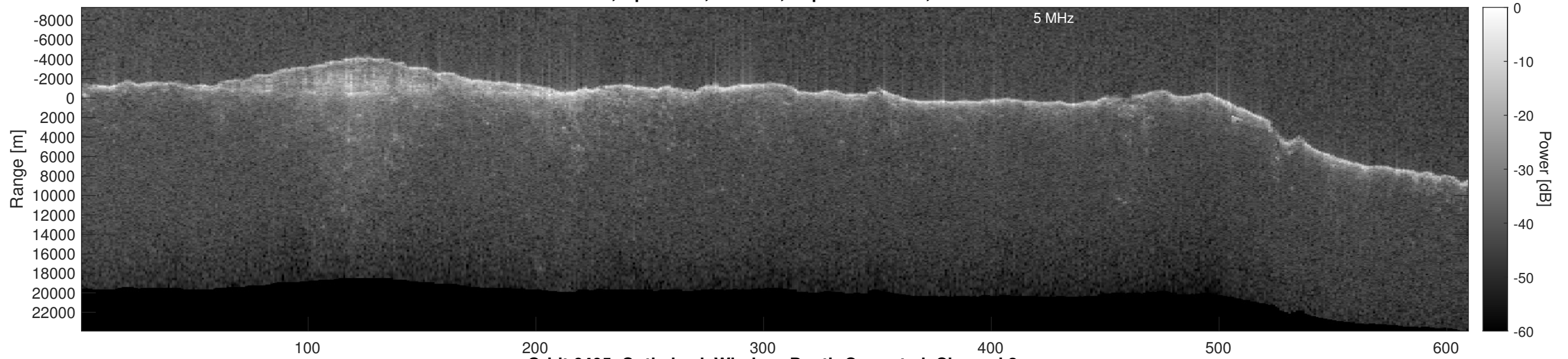
Orbit 6405, Optimized, Window, Depth-Corrected, Channel 2
