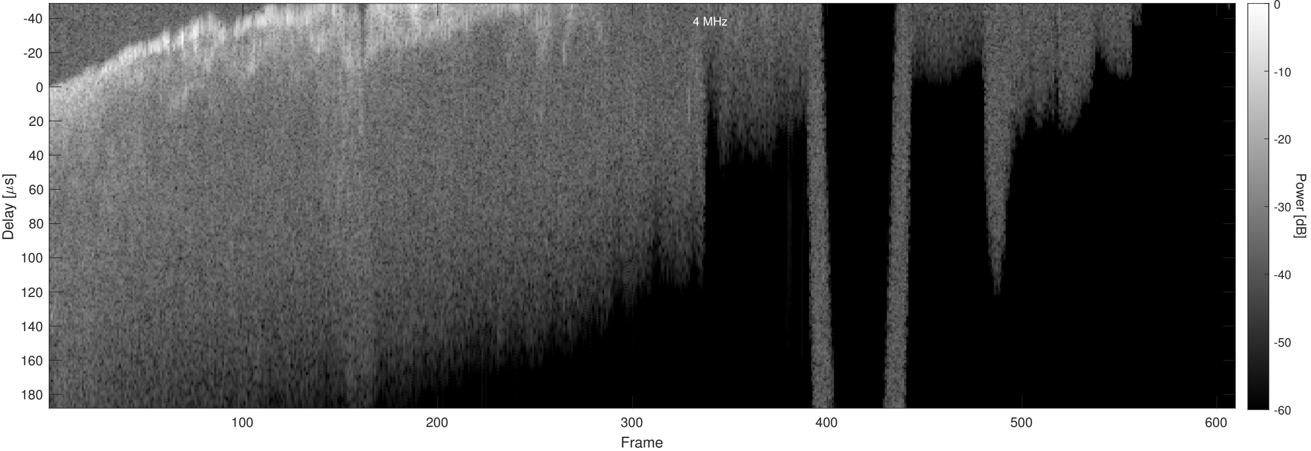
Orbit 6407, Chapman, Window, Channel 2
