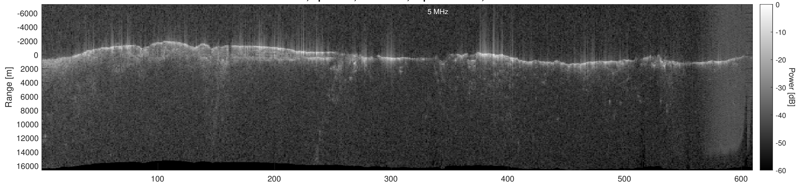
Orbit 6407, Optimized, No Window, Depth-Corrected, Channel 2
