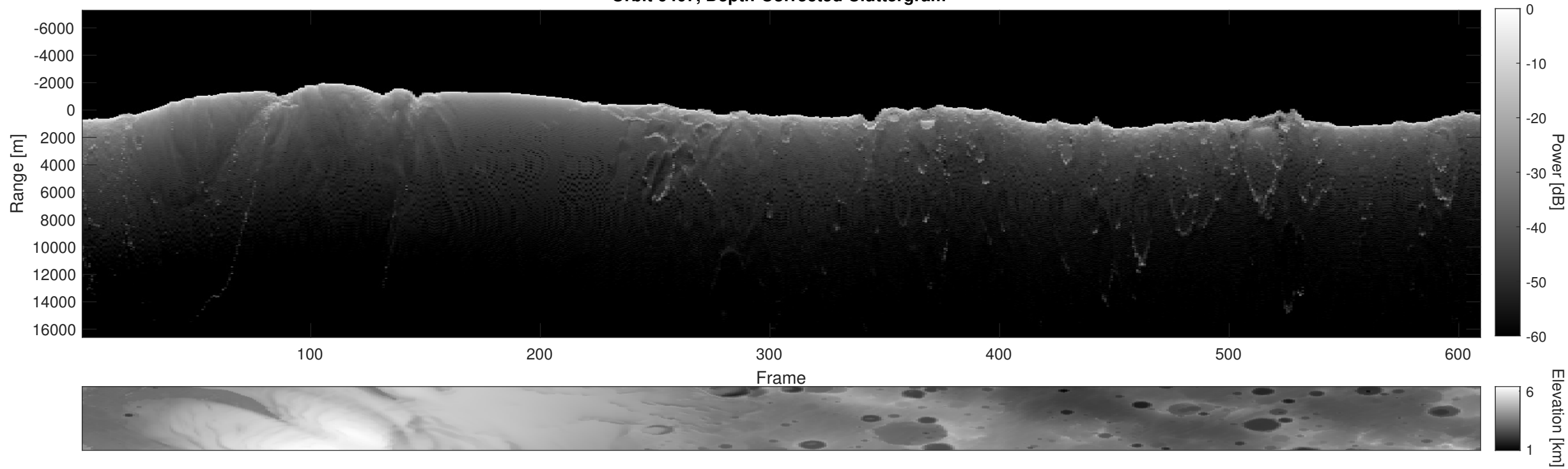
Orbit 6407, Depth-Corrected Cluttergram
