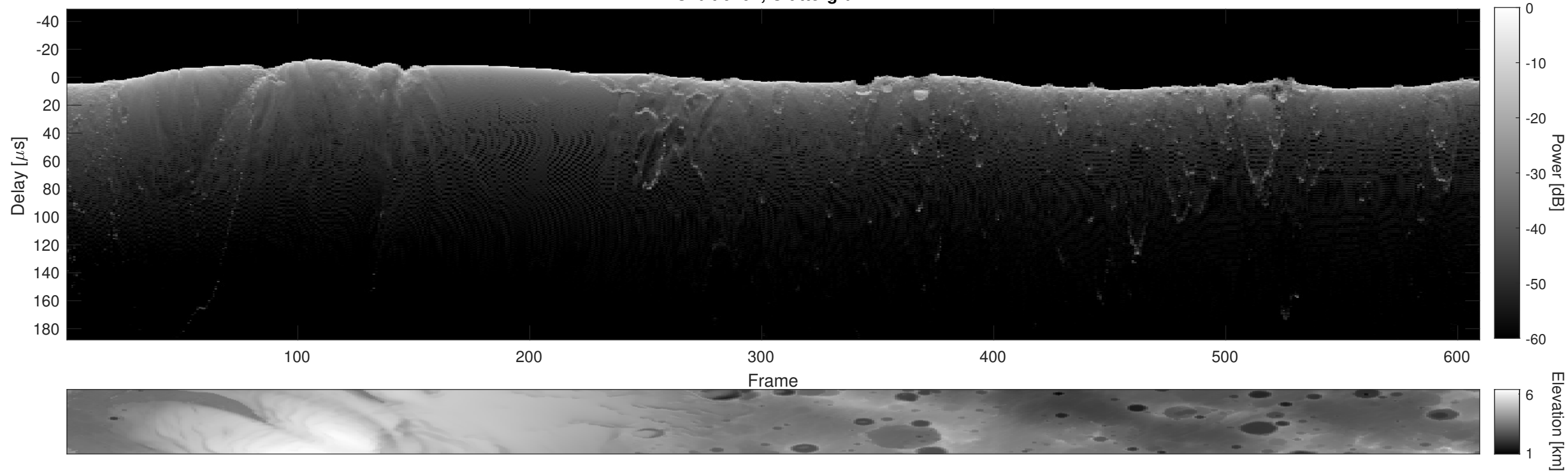
Orbit 6407, Cluttergram
