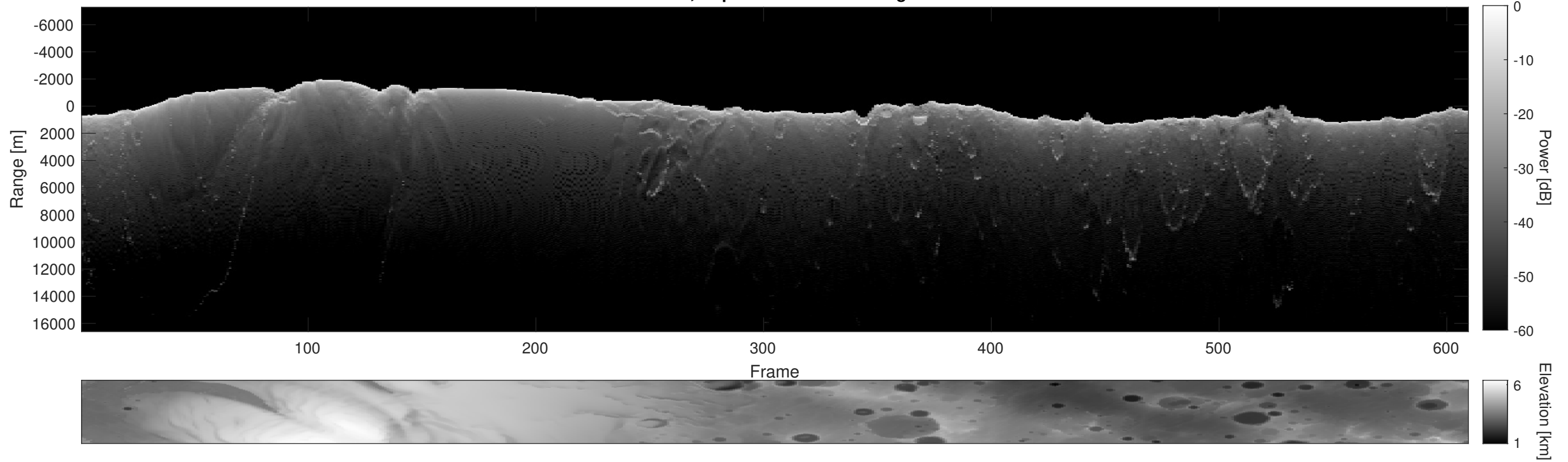
Orbit 6407, Depth-Corrected Cluttergram
