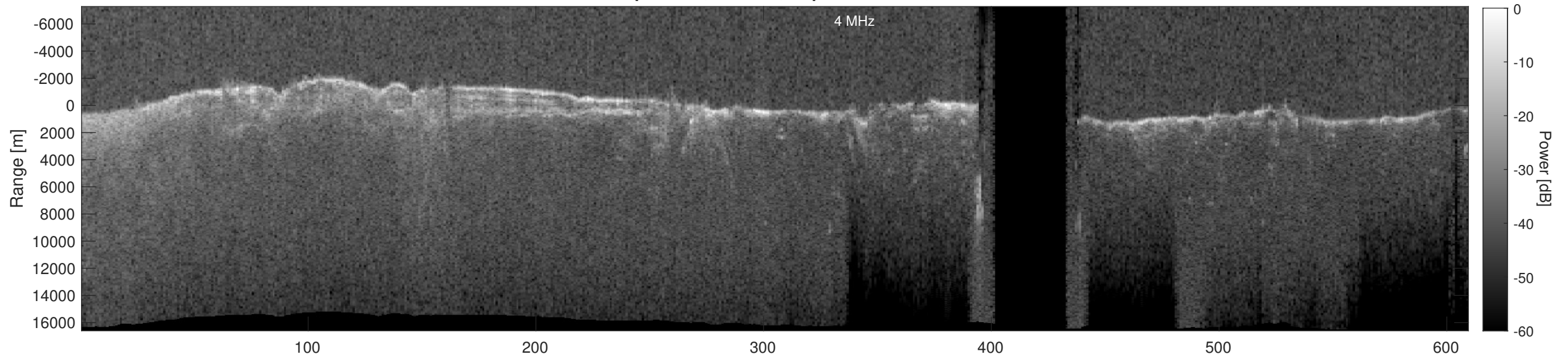
Orbit 6407, Depth-Corrected Cluttergram
