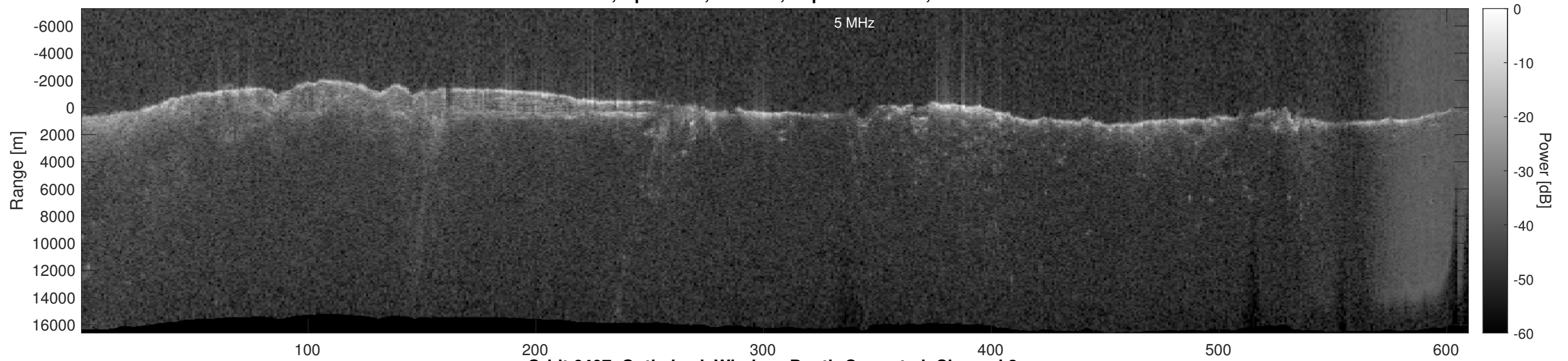
Orbit 6407, Optimized, Window, Depth-Corrected, Channel 2
