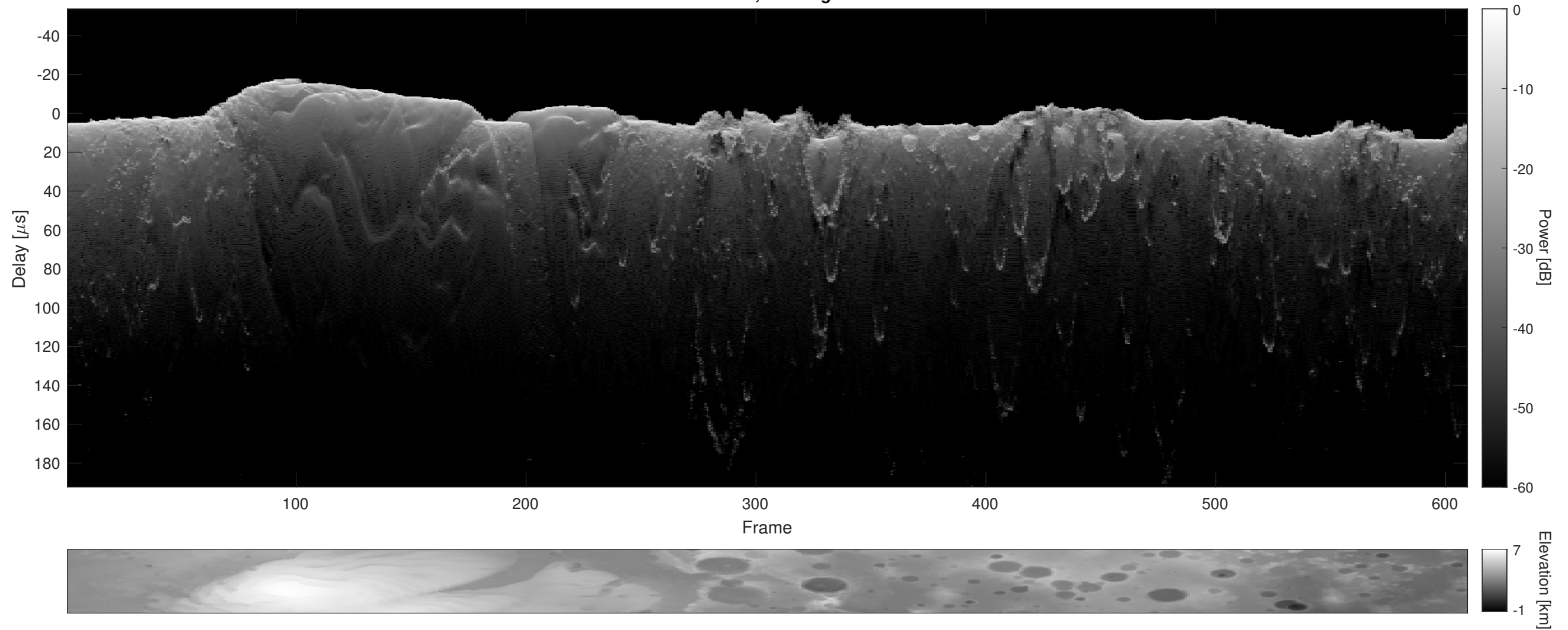
Orbit 6408, Cluttergram
