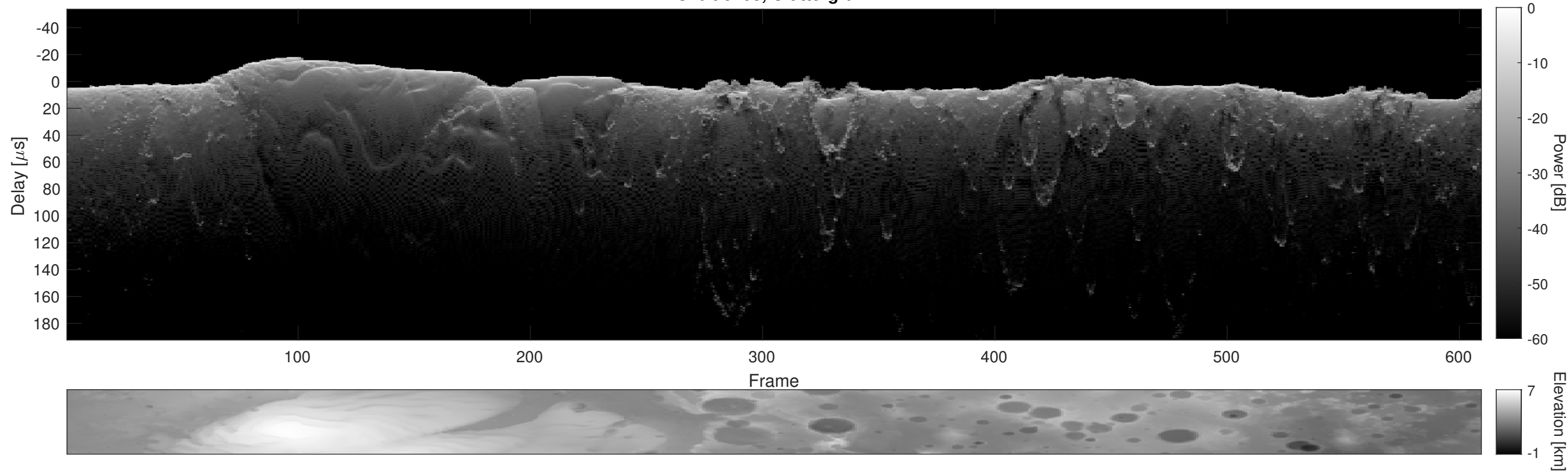
Orbit 6408, Cluttergram
