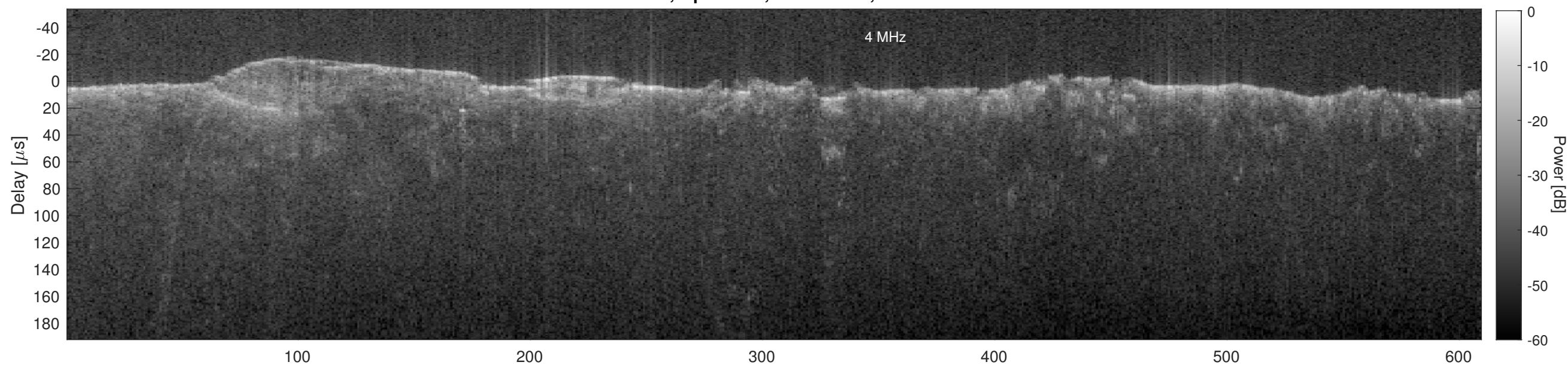
Orbit 6408, Cluttergram
