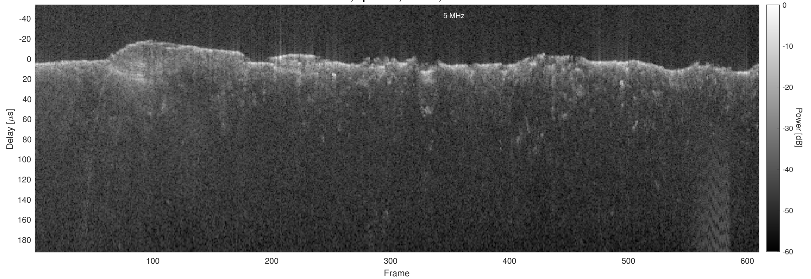
Orbit 6408, Optimized, Window, Channel 2
