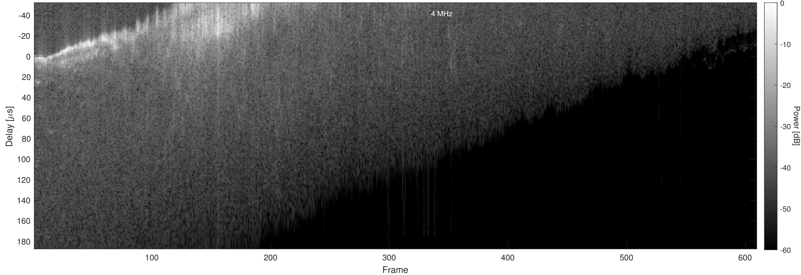
Orbit 6409, Chapman, No Window, Channel 2
