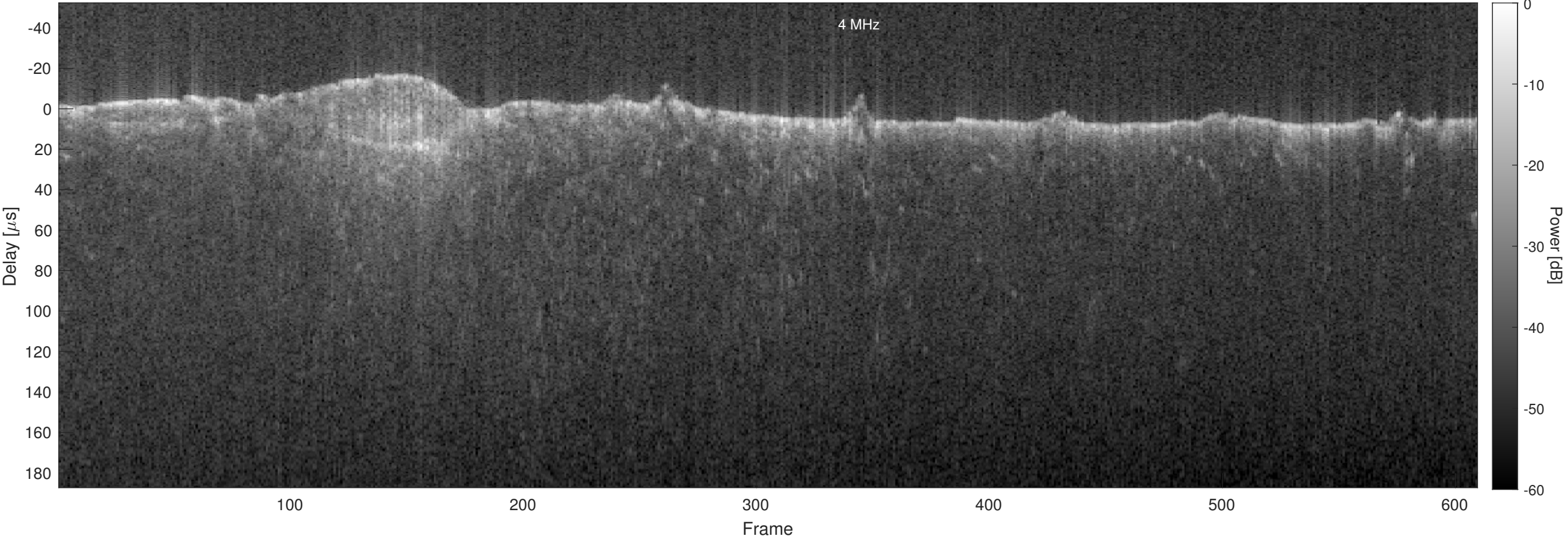
Orbit 6409, Optimized, No Window, Channel 2
