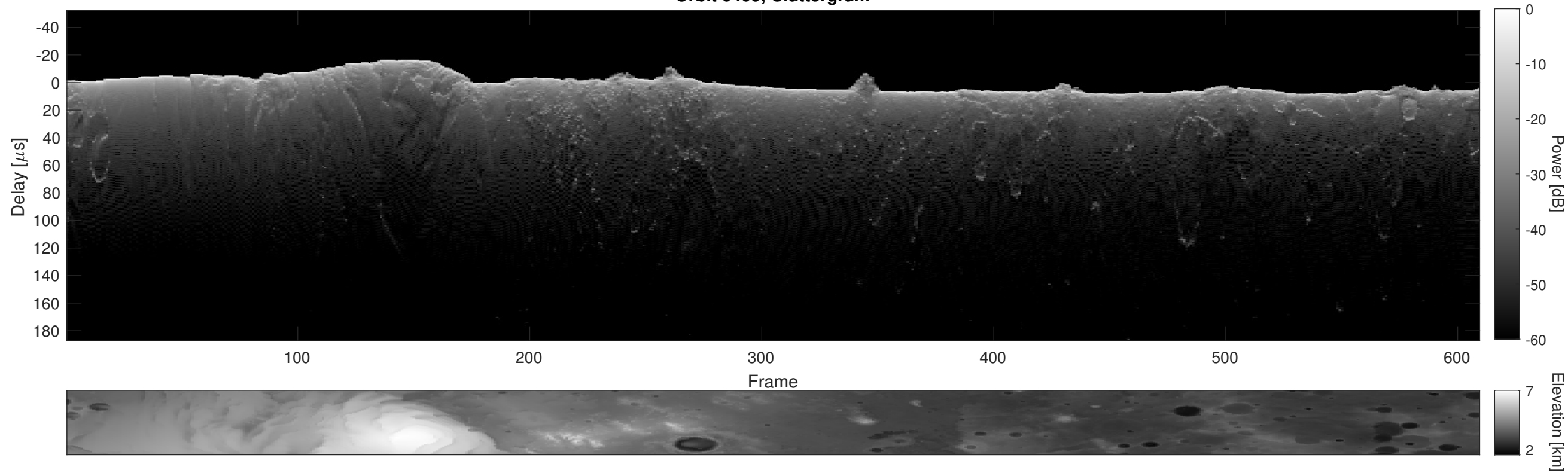
Orbit 6409, Cluttergram
