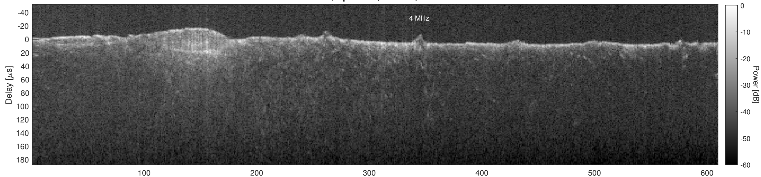
Orbit 6409, Cluttergram
