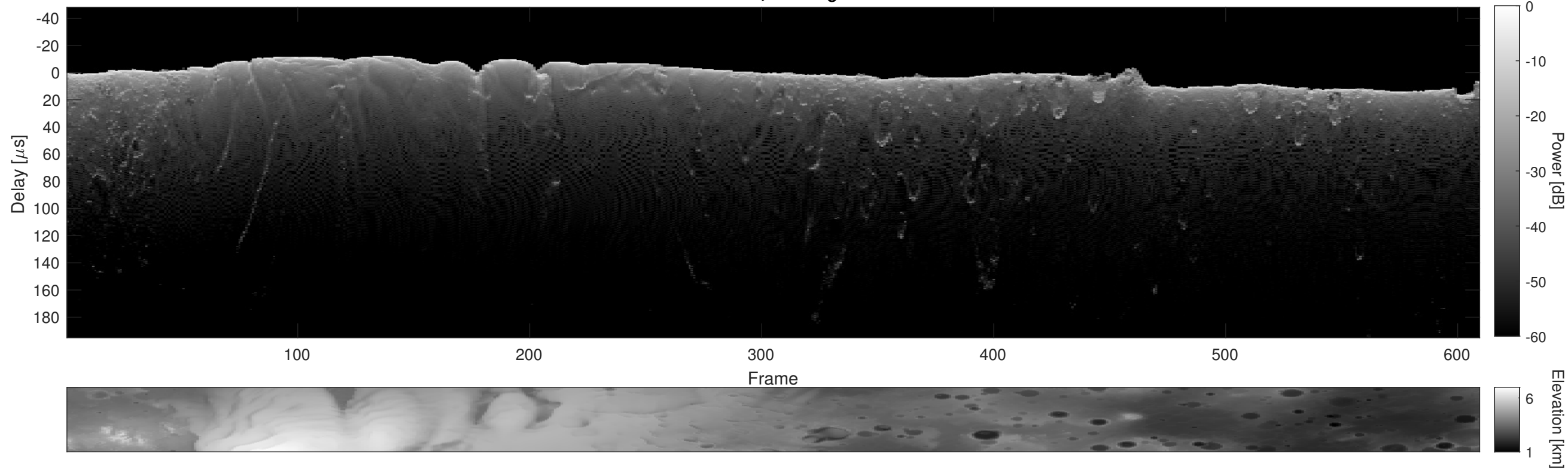
Orbit 6411, Cluttergram
