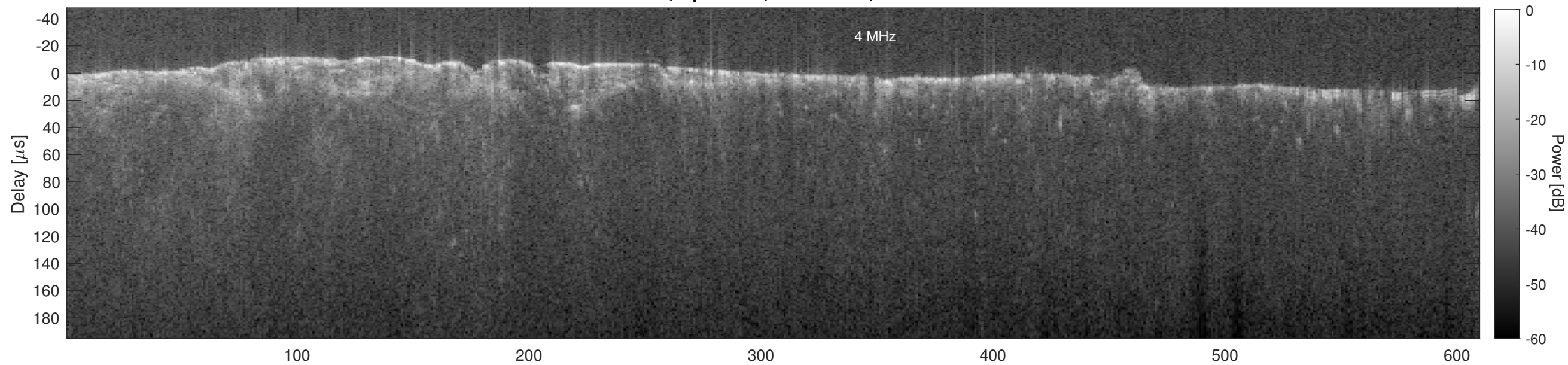
Orbit 6411, Cluttergram
