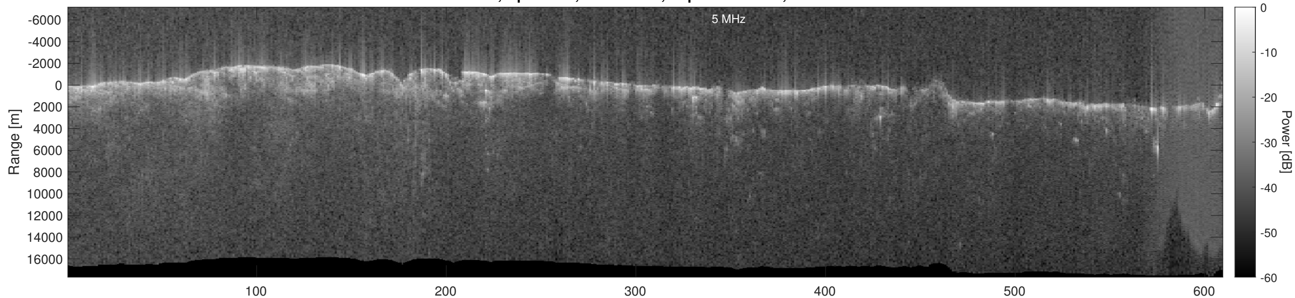
Orbit 6411, Optimized, No Window, Depth-Corrected, Channel 2
