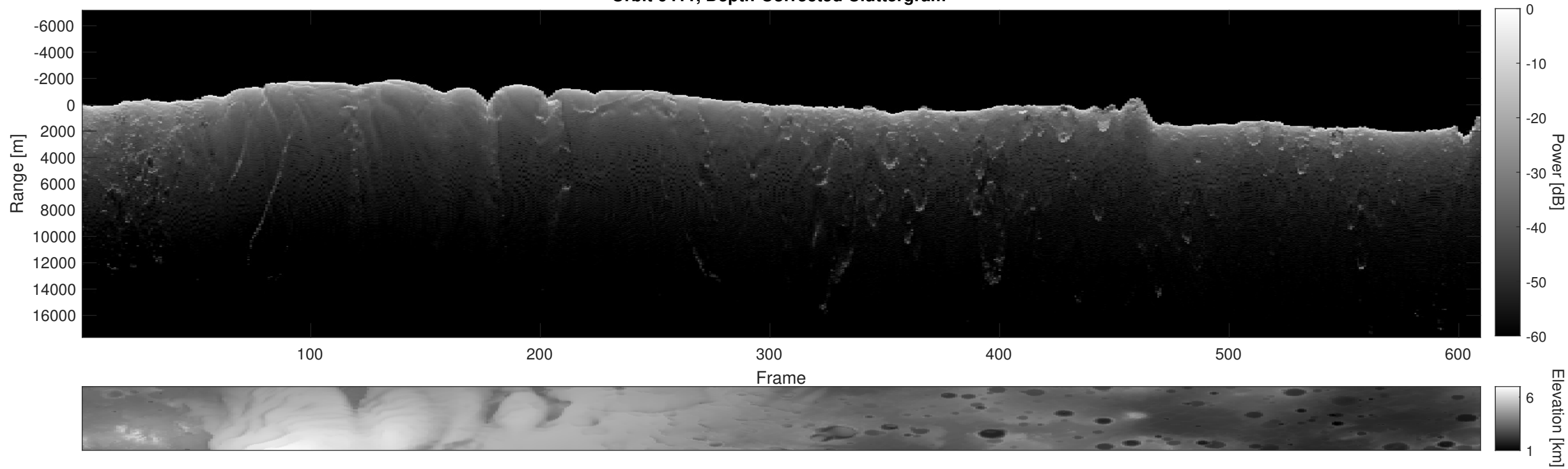
Orbit 6411, Depth-Corrected Cluttergram
