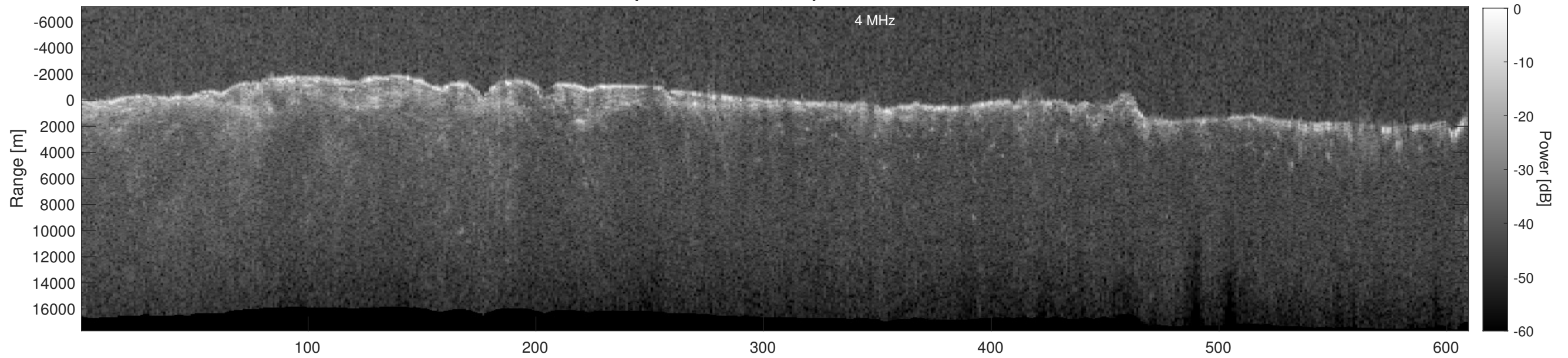
Orbit 6411, Depth-Corrected Cluttergram
