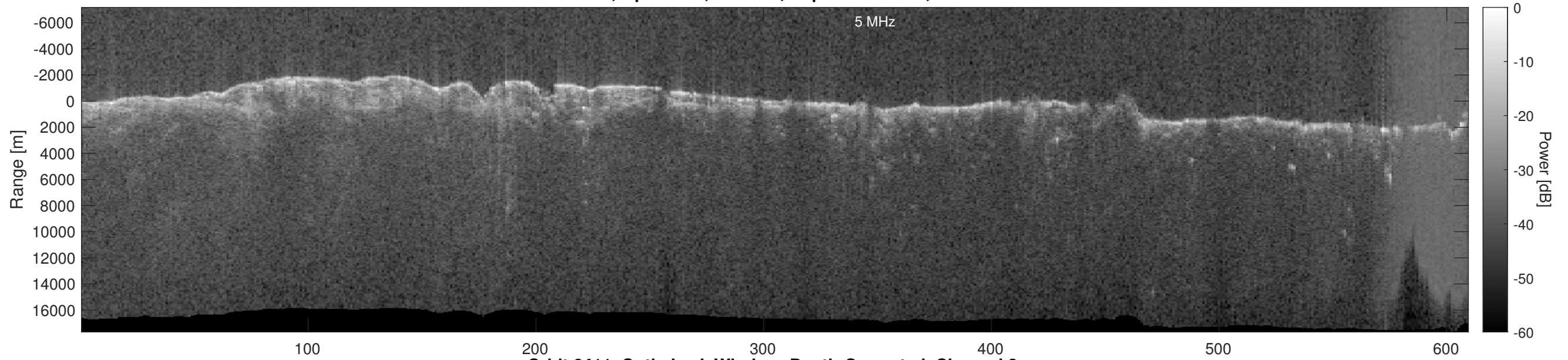
Orbit 6411, Optimized, Window, Depth-Corrected, Channel 2
