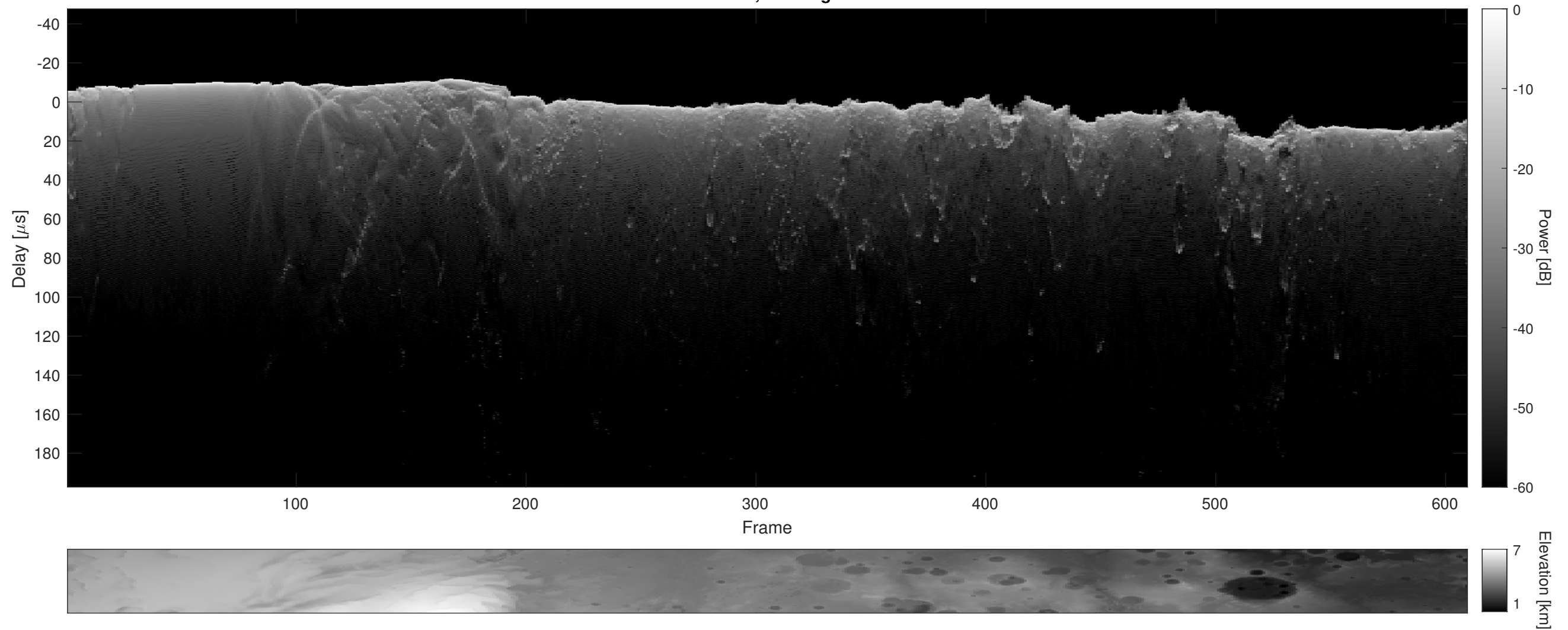
Orbit 6413, Cluttergram
