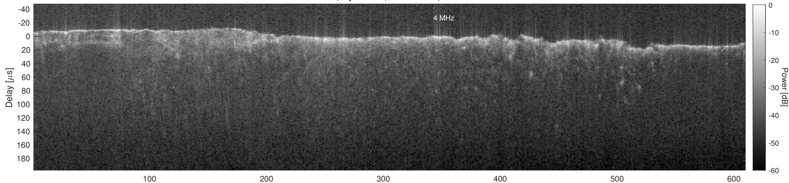
Orbit 6413, Cluttergram
