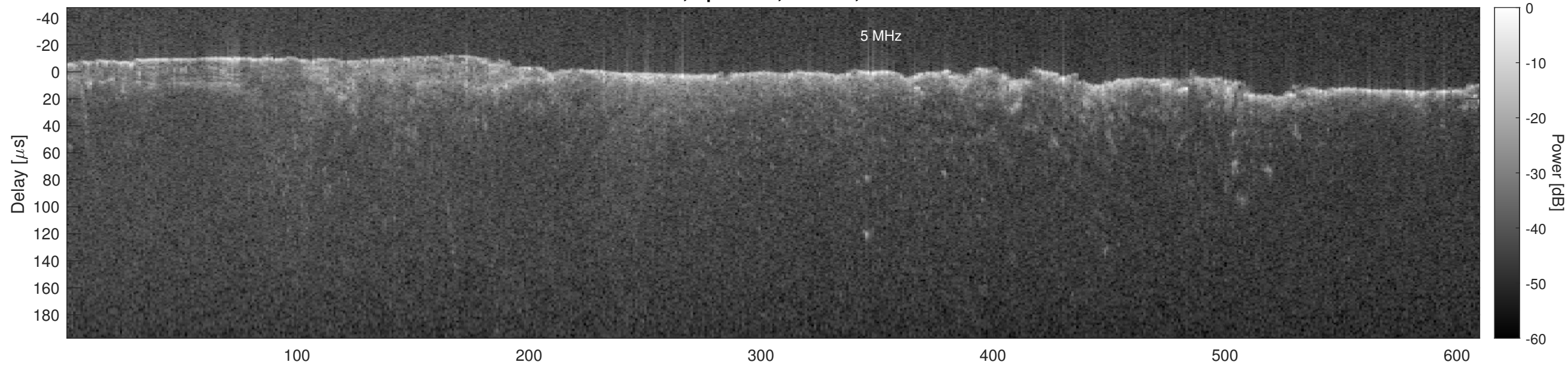
Orbit 6413, Optimized, Window, Channel 2
