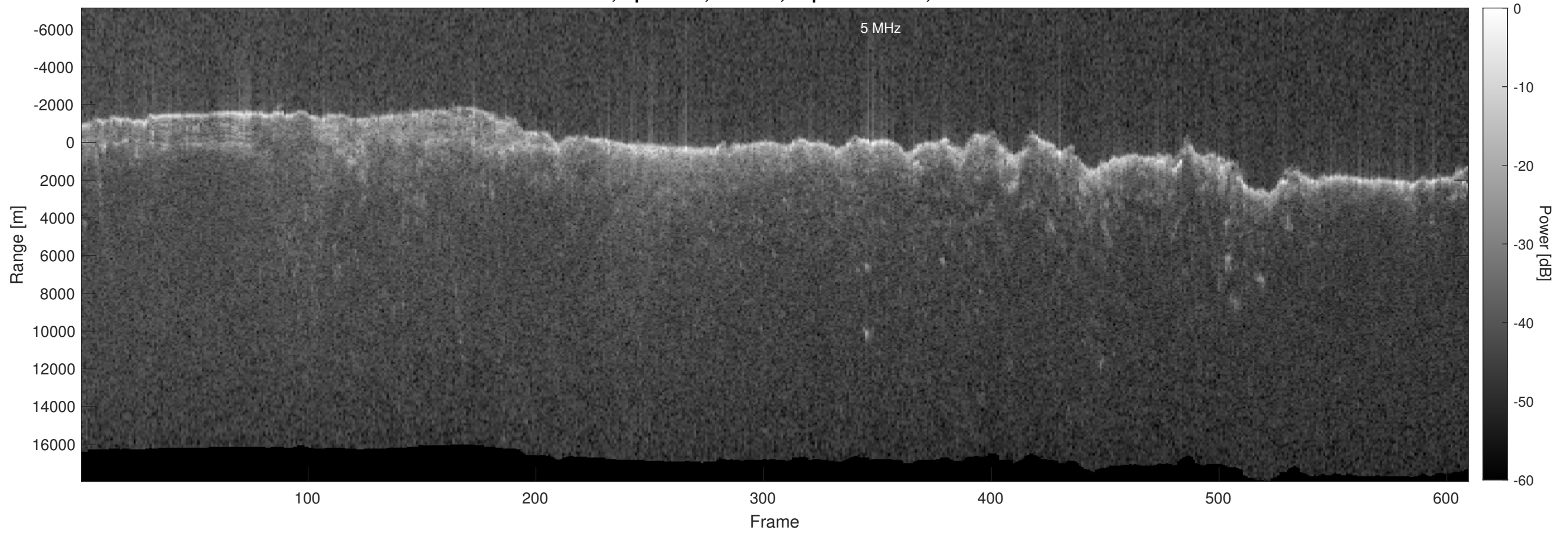
Orbit 6413, Optimized, Window, Depth-Corrected, Channel 2
