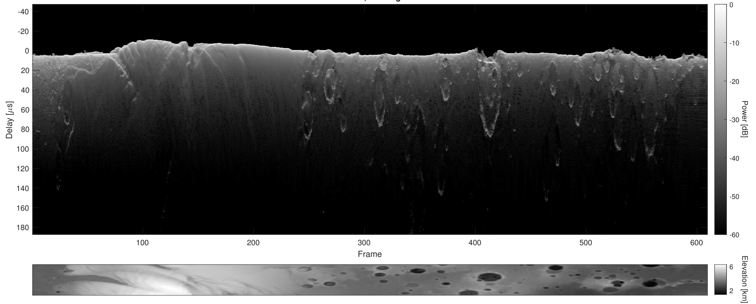
Orbit 6414, Cluttergram
