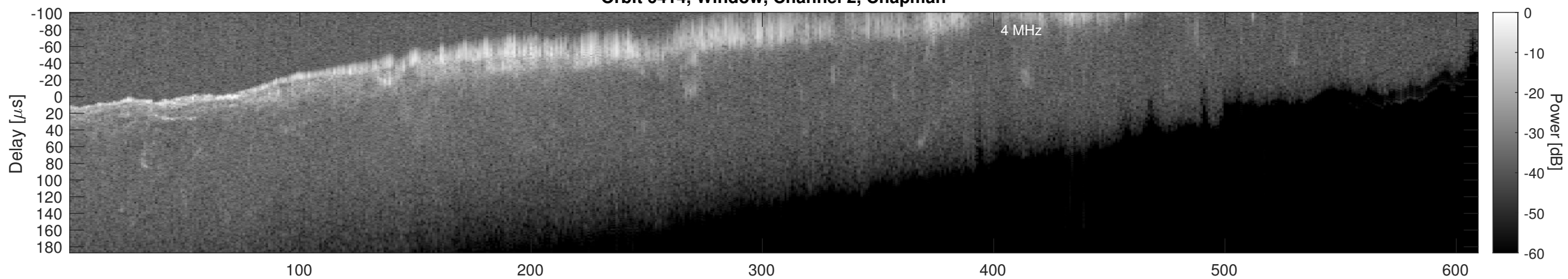
Orbit 6414, Window, Channel 2, Optimized
