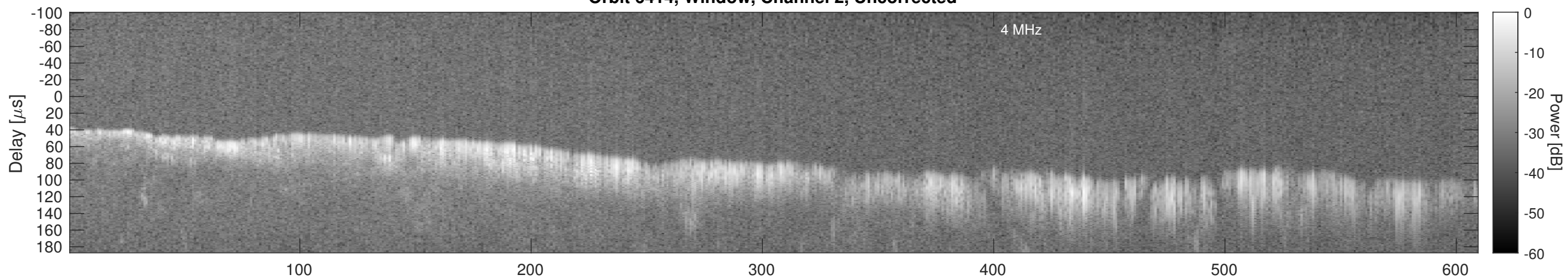
Orbit 6414, Window, Channel 2, Chapman
