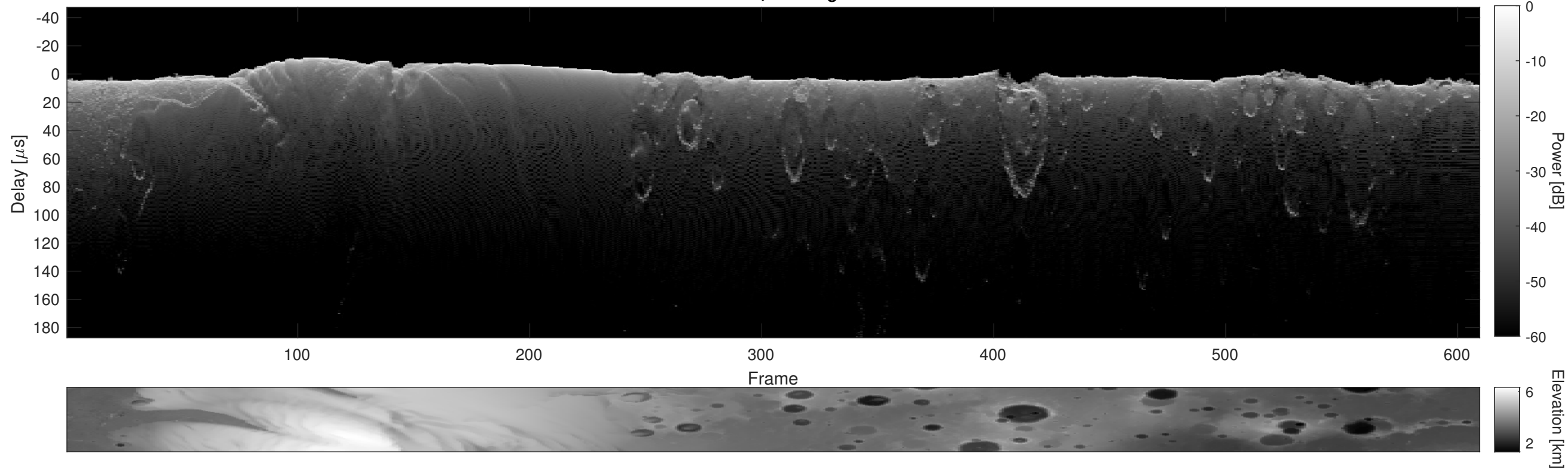
Orbit 6414, Cluttergram
